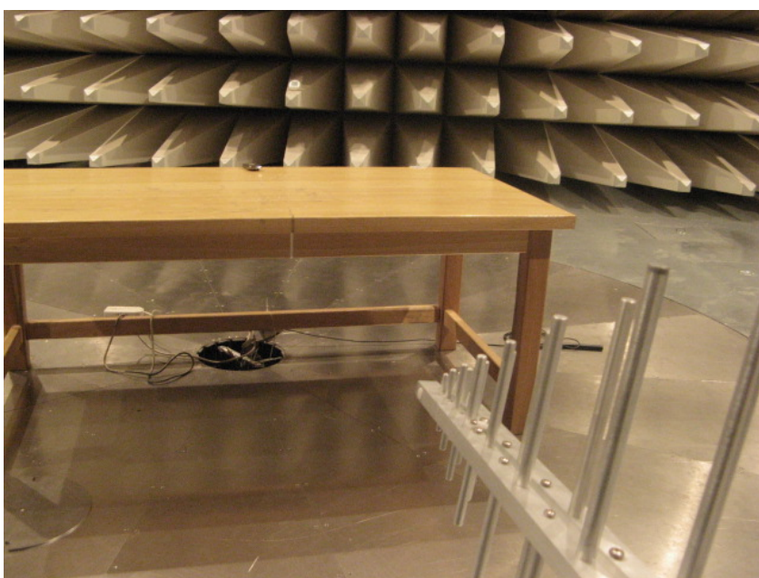
Picture 3 Radiated emission 15C
