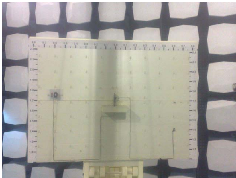
Picture 1 RF output power measurement and Band Edge compliance
