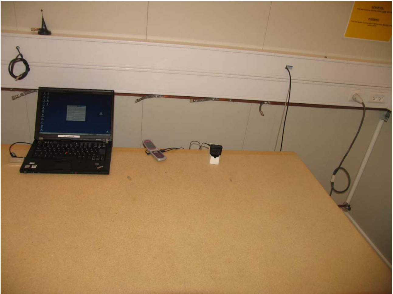
Picture 3 AC powerline conducted emission measurement 15B
