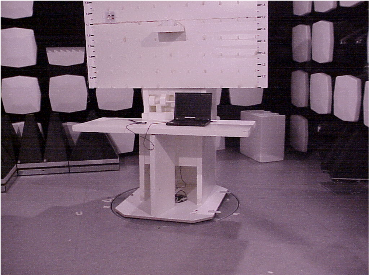
Picture 1 Radiated Emission 15B
