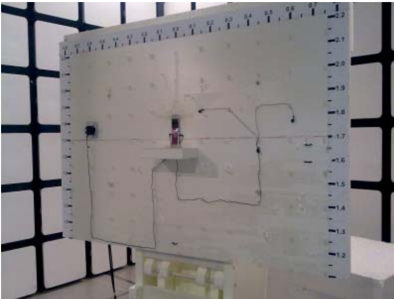
Picture 1 Radiated emission 15C
