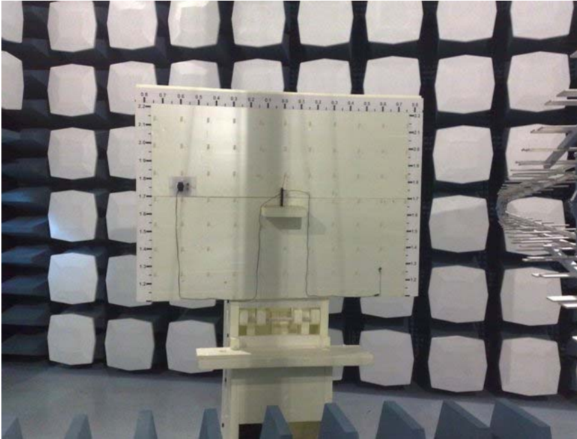
Picture 1 RF output power measurement and Band Edge measurement
