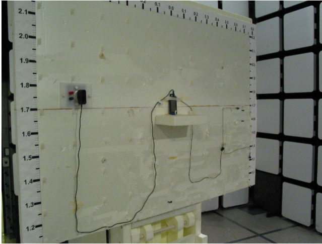
Picture 1. FCC Part 15C Radiated emissions
