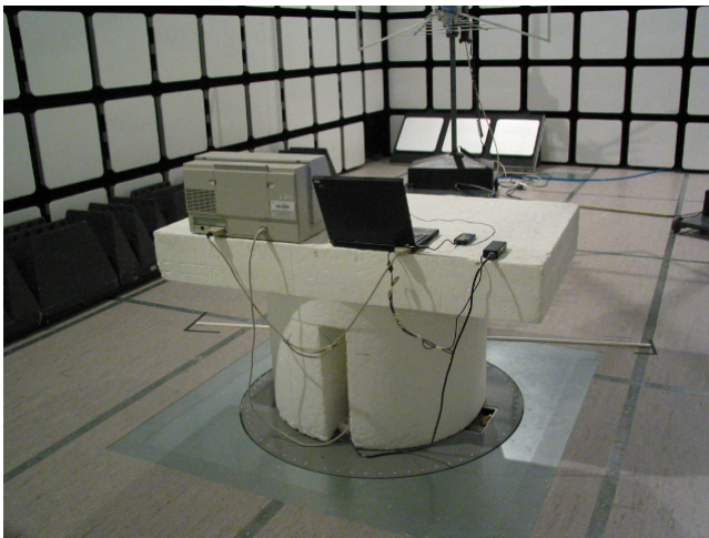
Picture 2. FCC Part 15B Radiated emissions
