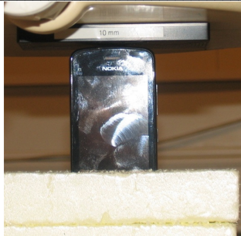
Photo of the device positioned for WR mode measurement – top edge facing phantom. The spacer was removed before the start of the measurements.
