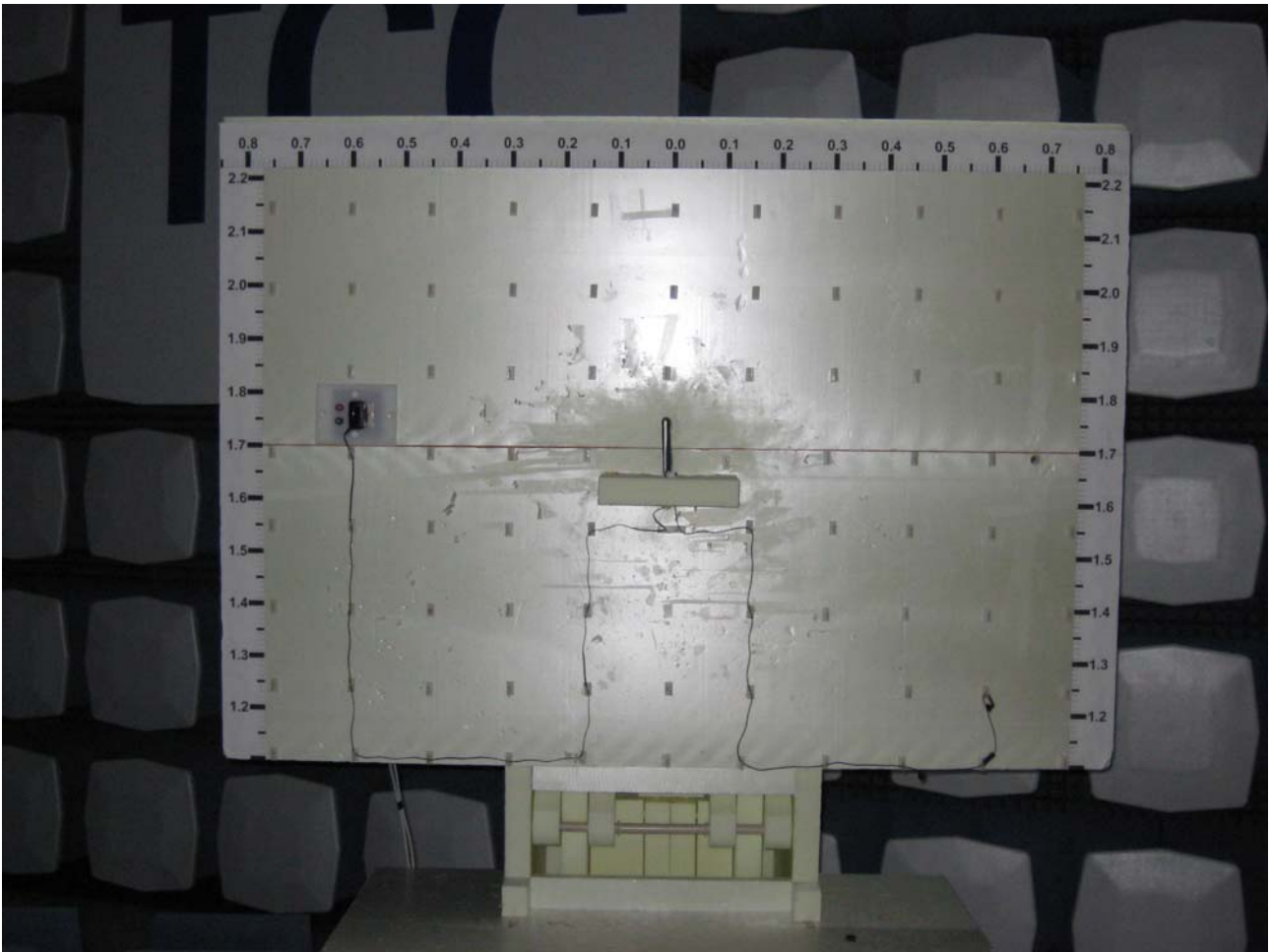
Picture 1 Spurious radiated emission measurement
