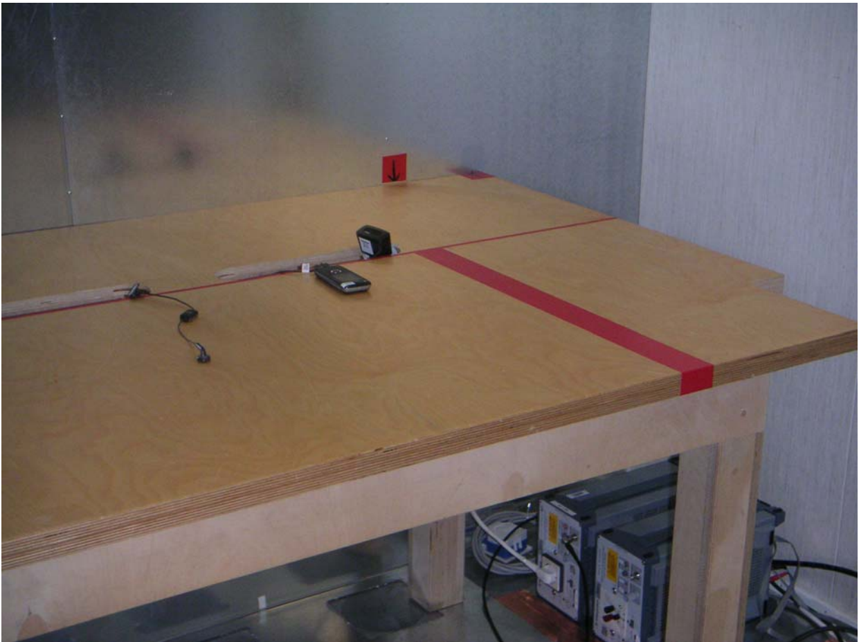
Picture 4 AC powerline conducted emission measurement Bluetooth TX / WLAN TX
