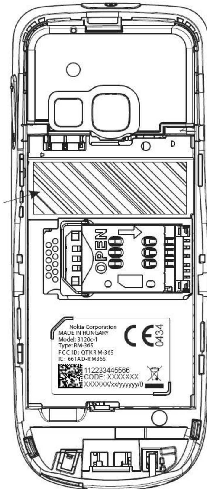
RM-365 FCC Label and location
