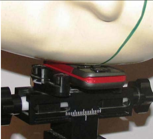
Photo of the device in "cheek" position with slide closed
