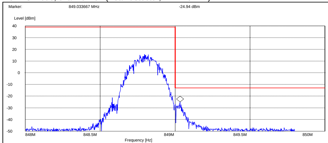
EGPRS mode, channel 251 (Peak detector, RBW: 3 kHz)
