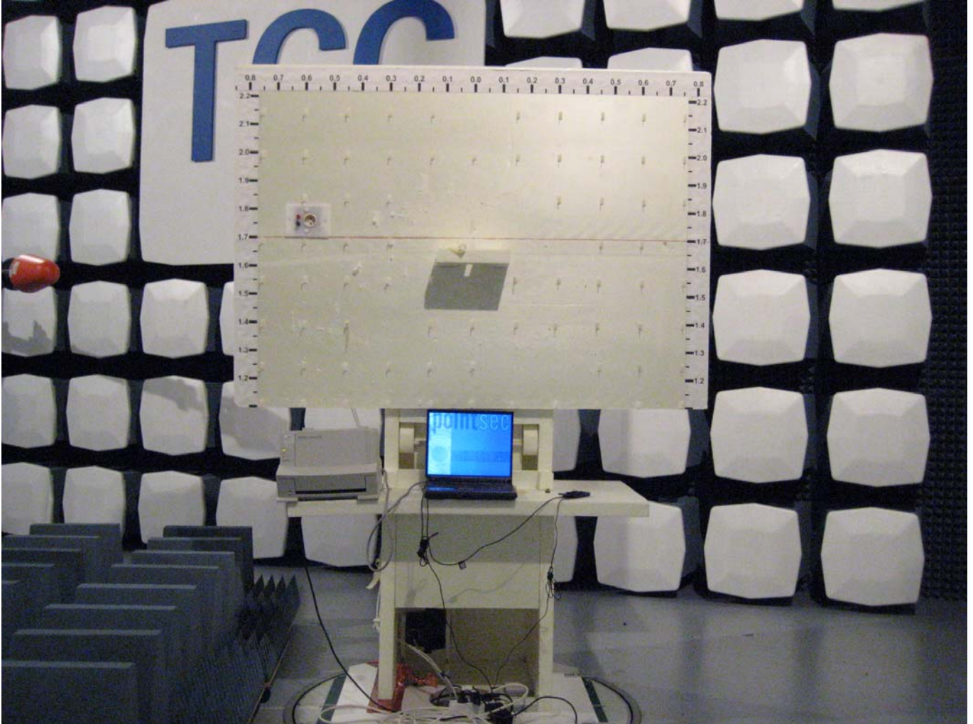
Picture 2 Radiated emission measurement + Computer peripherals
