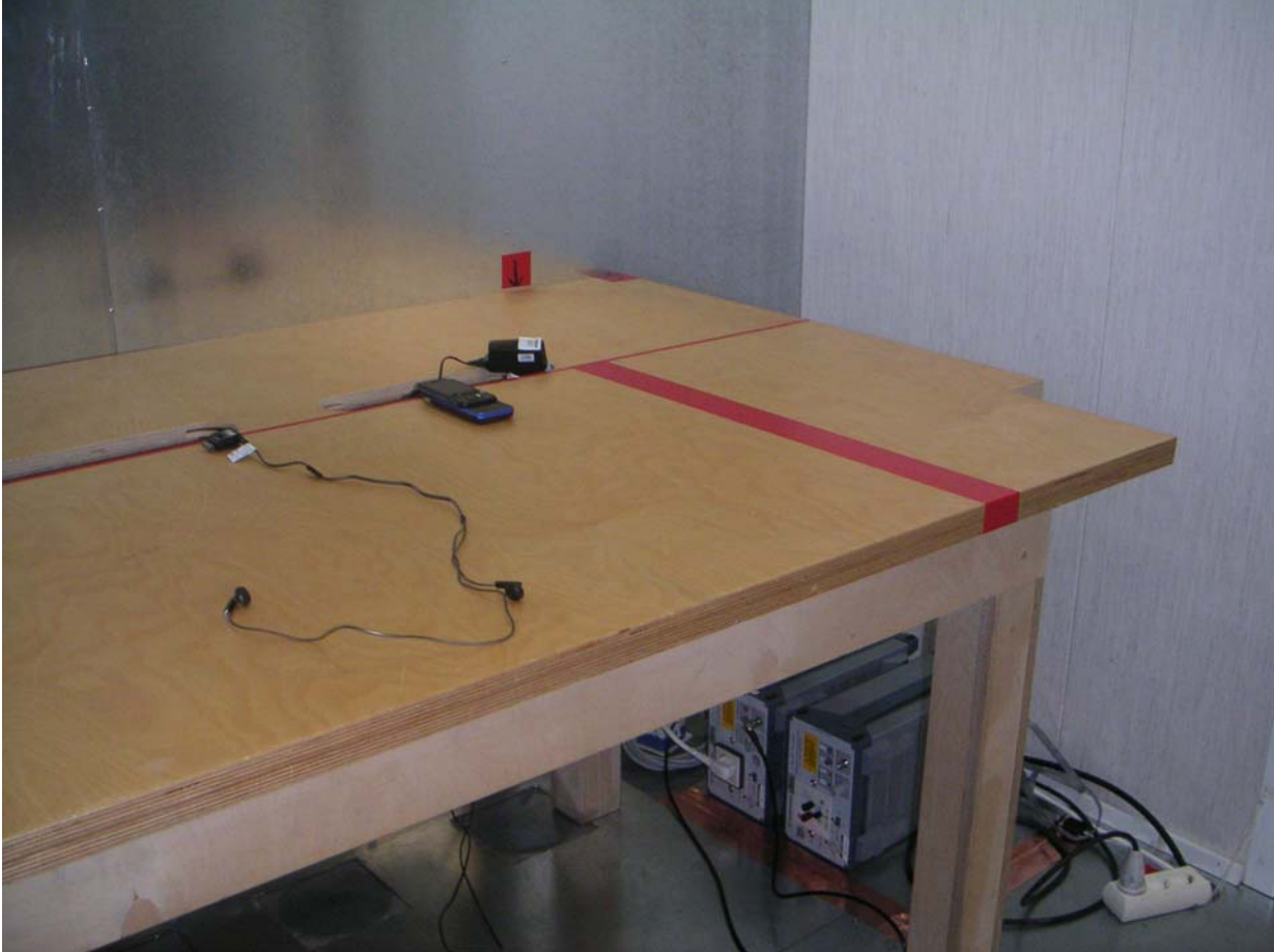
Picture 3 AC powerline conducted emission measurement
