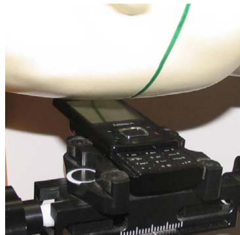
Photo of the device open in "tilt" position
