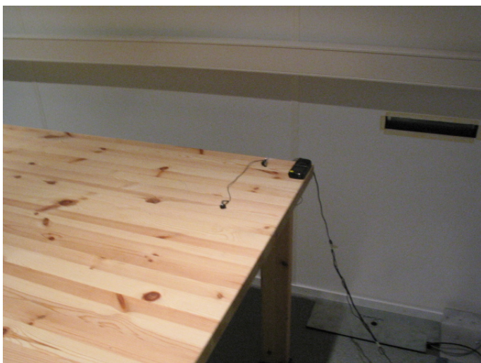
Picture 4 AC powerline conducted emission measurement Bluetooth TX
