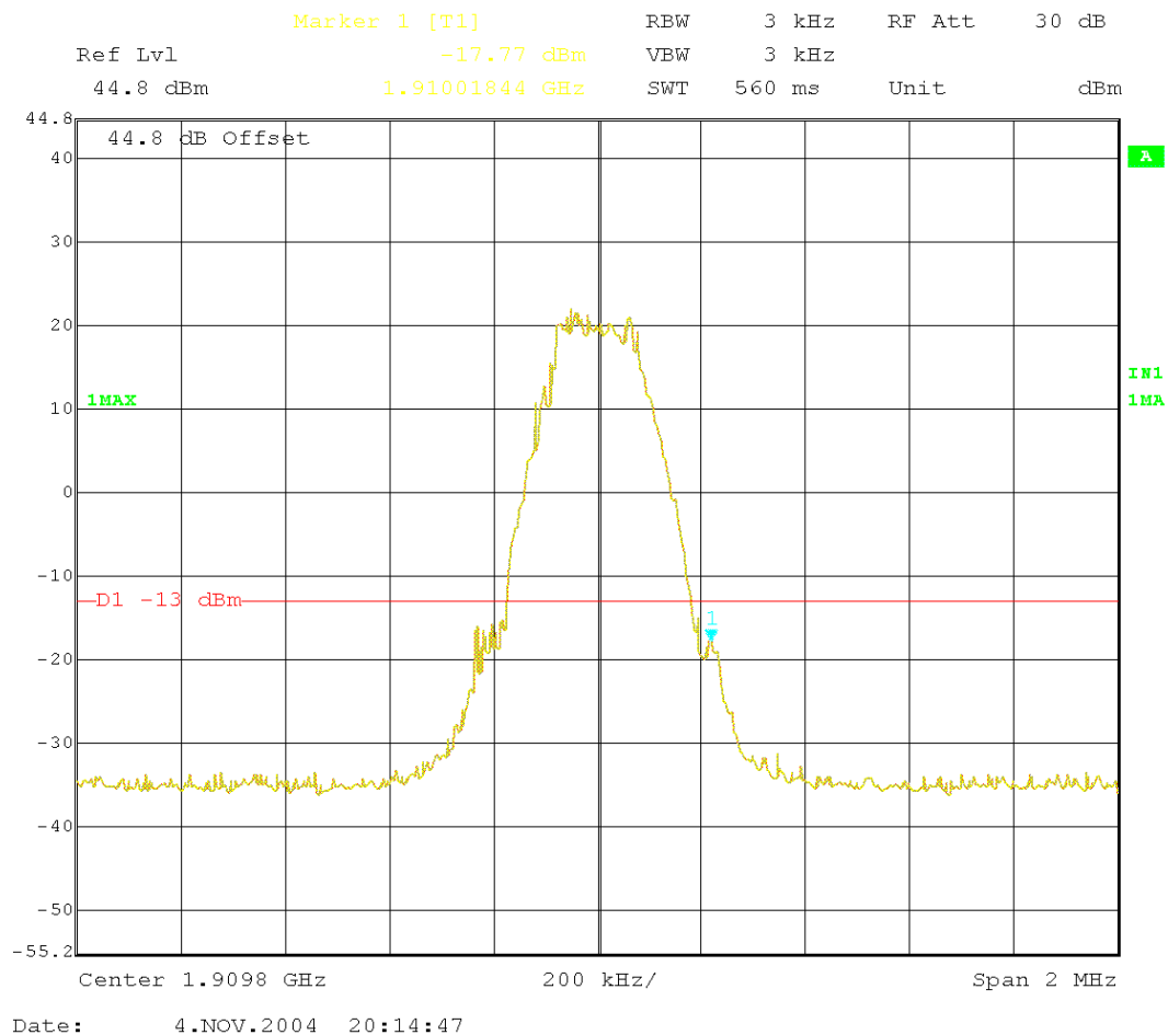
Picture 8. Upper bandedge E-GPRS, channel 810, RBw 3KHz VBw 3KHz
