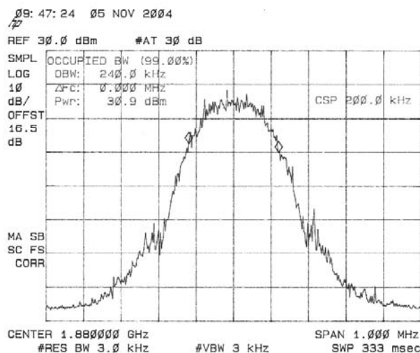
Picture 4. 99% occupied bandwidth, channel 661, GSM
