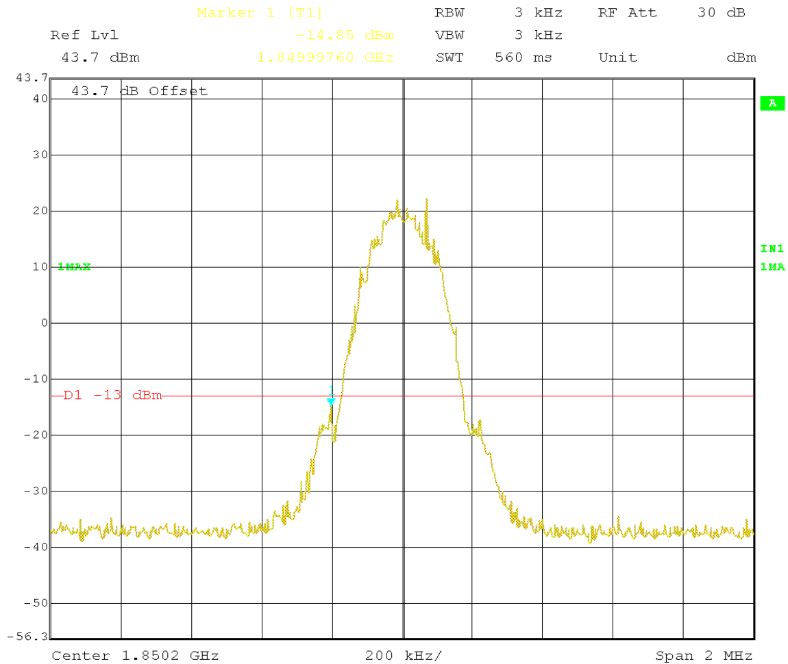
Picture 5. Lower bandedge GSM/GPRS, channel 512, RBw 3KHz VBw 3KHz
