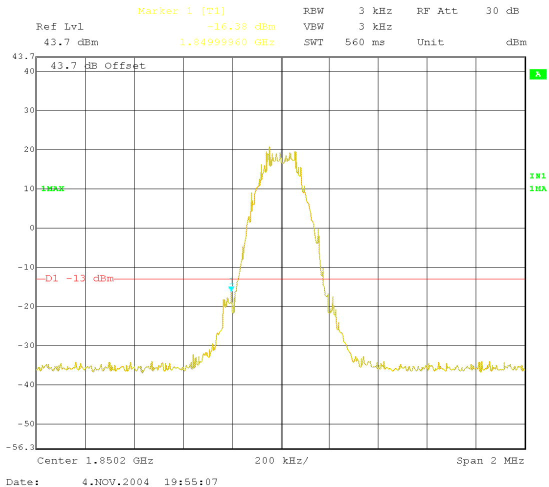
Picture 7. Lower bandedge E-GPRS, channel 512, RBw 3KHz VBw 3KHz
