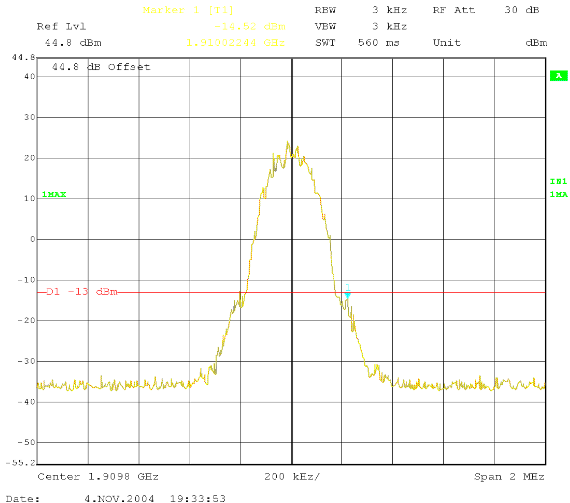
Picture 6. Upper bandedge GSM/GPRS, channel 810, RBw 3KHz VBw 3KHz
