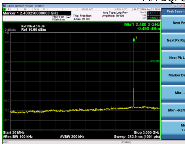
Pi/4 DQPSK High Channel
