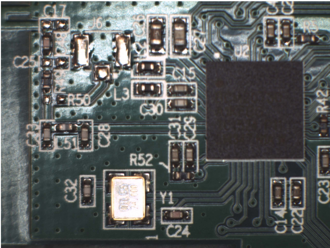
Figure 1 - RF Area Top of PCBA
