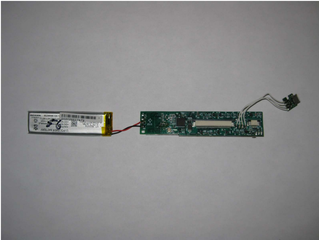
Figure 3 - Top of LMA with battery
