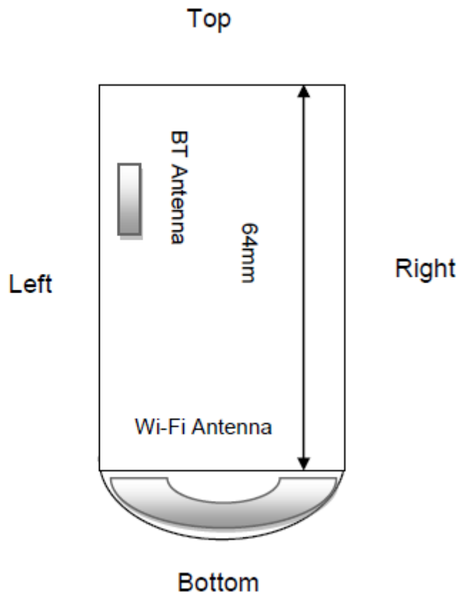
(78mm*45mm)Front view:
