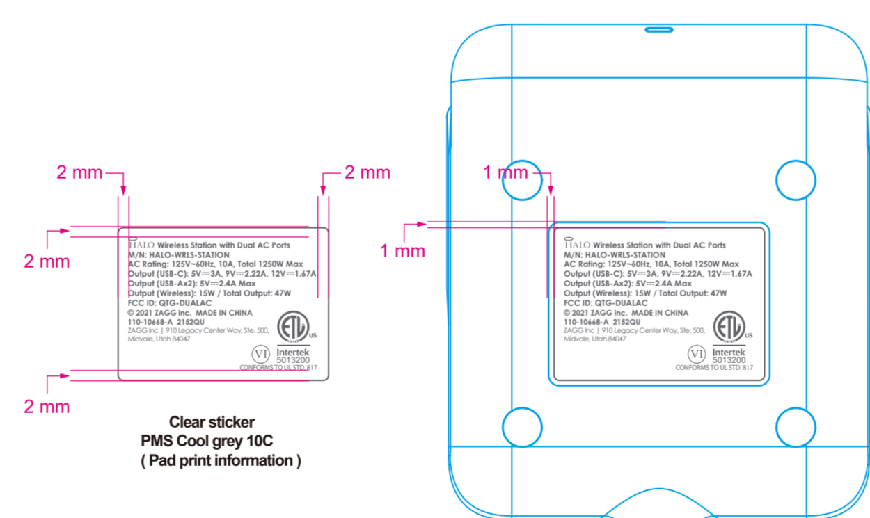
Bottom view
