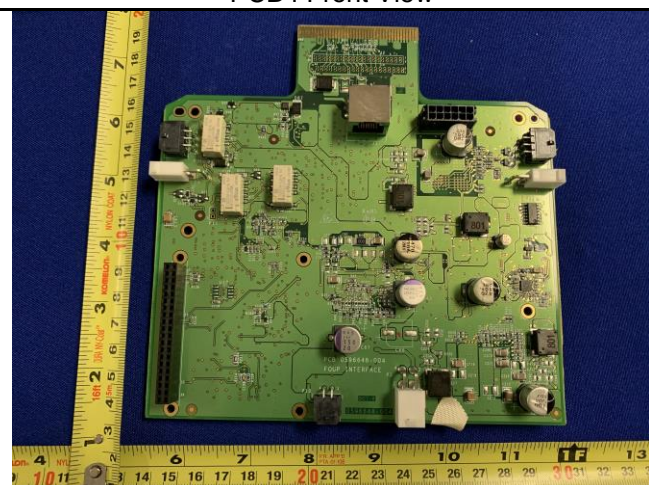
PCB5 Front View
