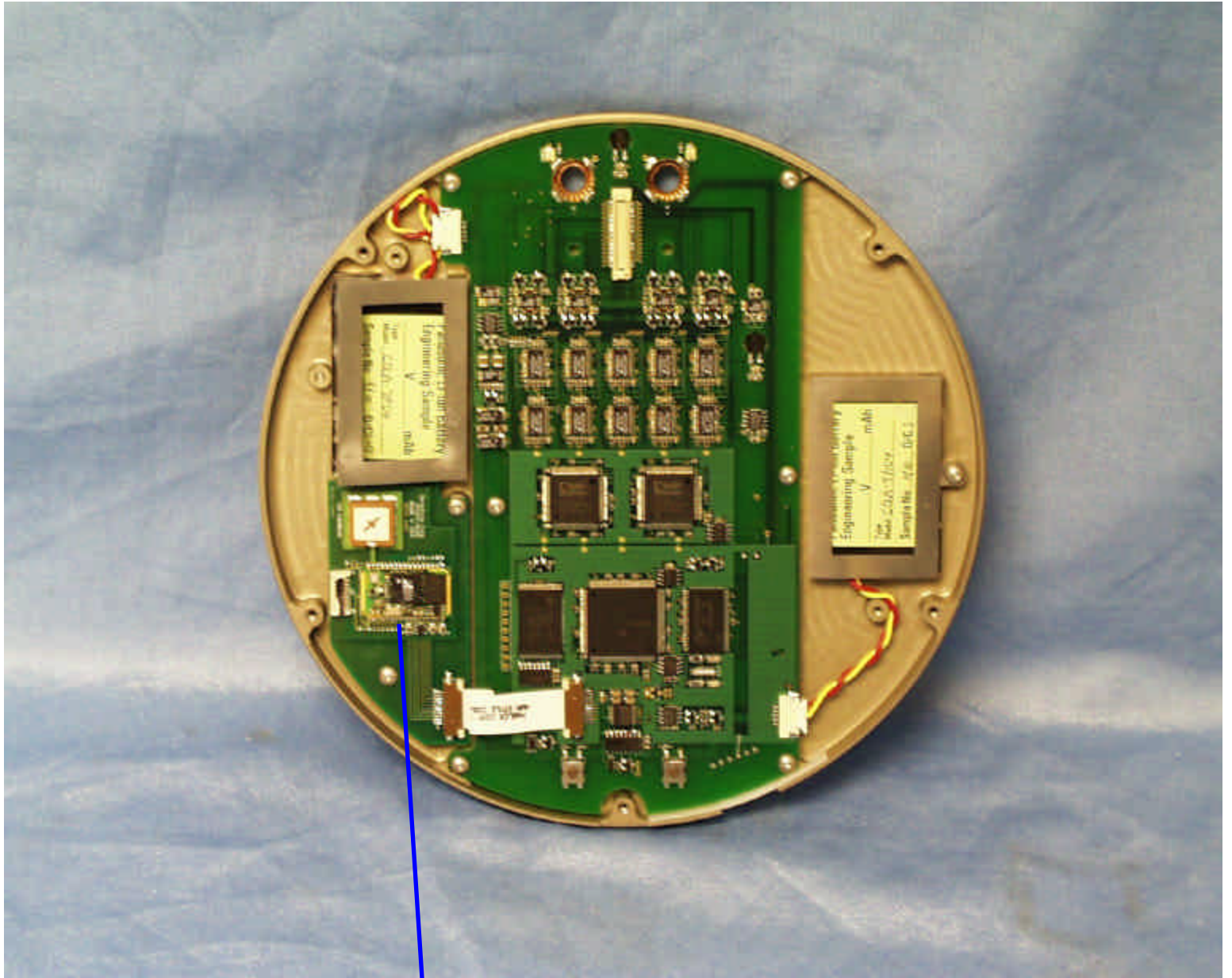
Bluetooth Radio
