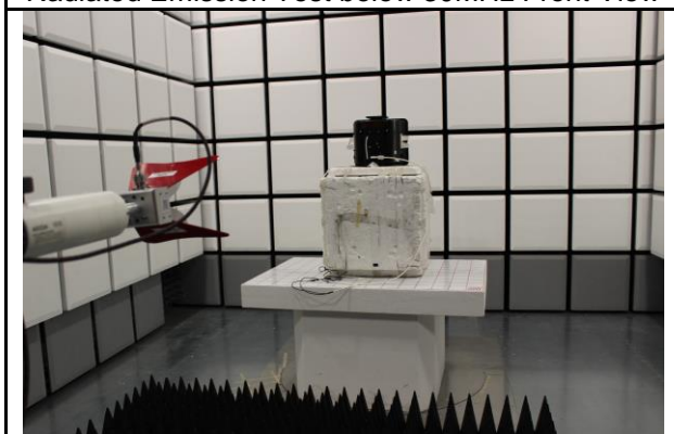
Radiated Emission Test below 1GHz Front View
