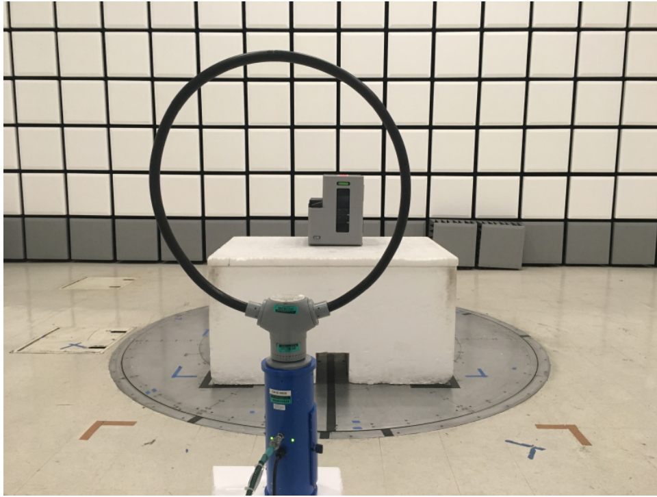
Radiated Spurious Emissions Below 30 MHz Front
