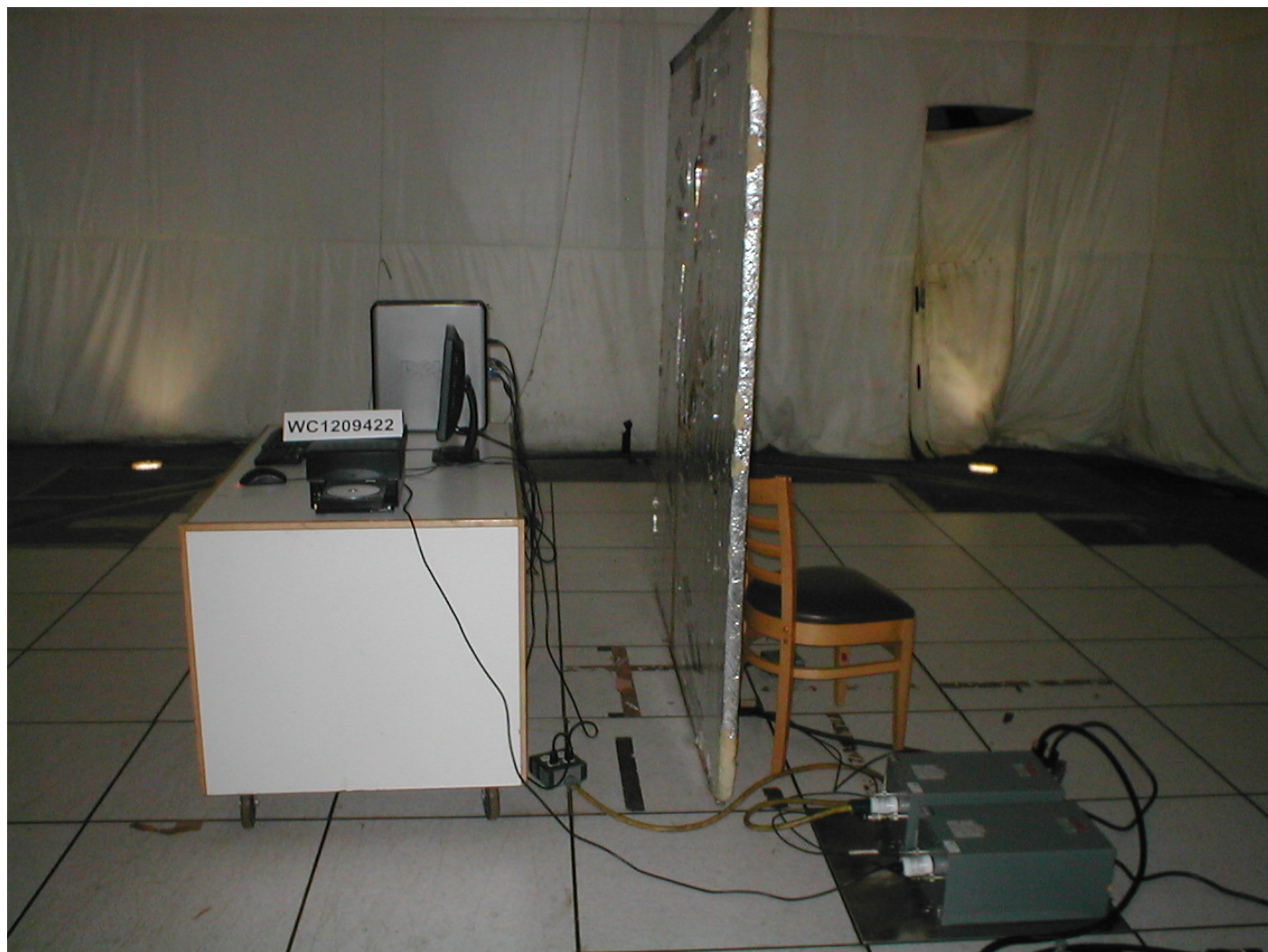
Test-setup photo(s):
