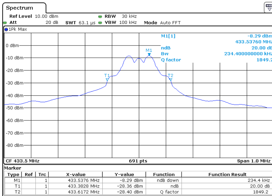
Channel 01: 433.50MHz
