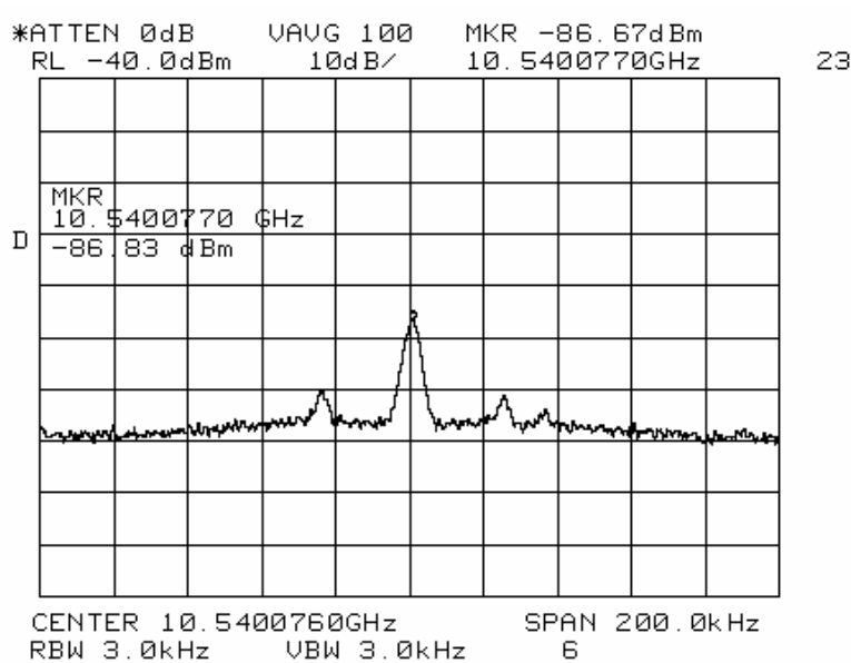
Plot 3: Second Harmonic, 3kHz RBW:
