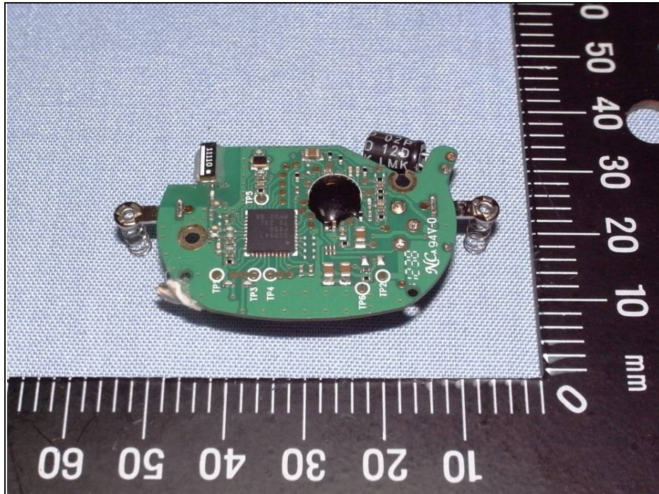
PCB
