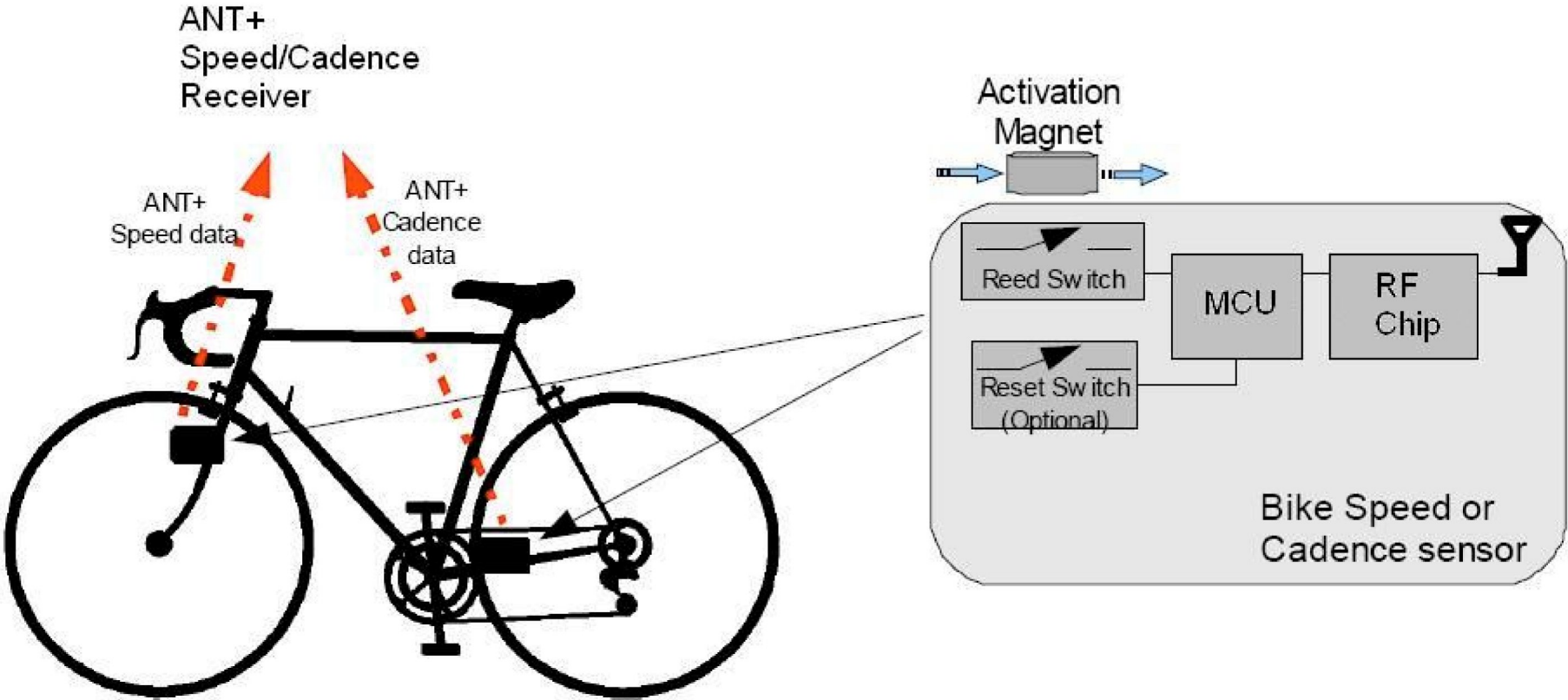
Typical installation of sensor modules for speed and cadence sensing.
