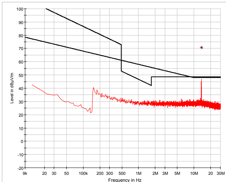
— EN 300 330 tx mag — FCC 15.209 mag (10 m) — MaxPeak-ClearWrite-PK+ * Final Result 1-QPK
