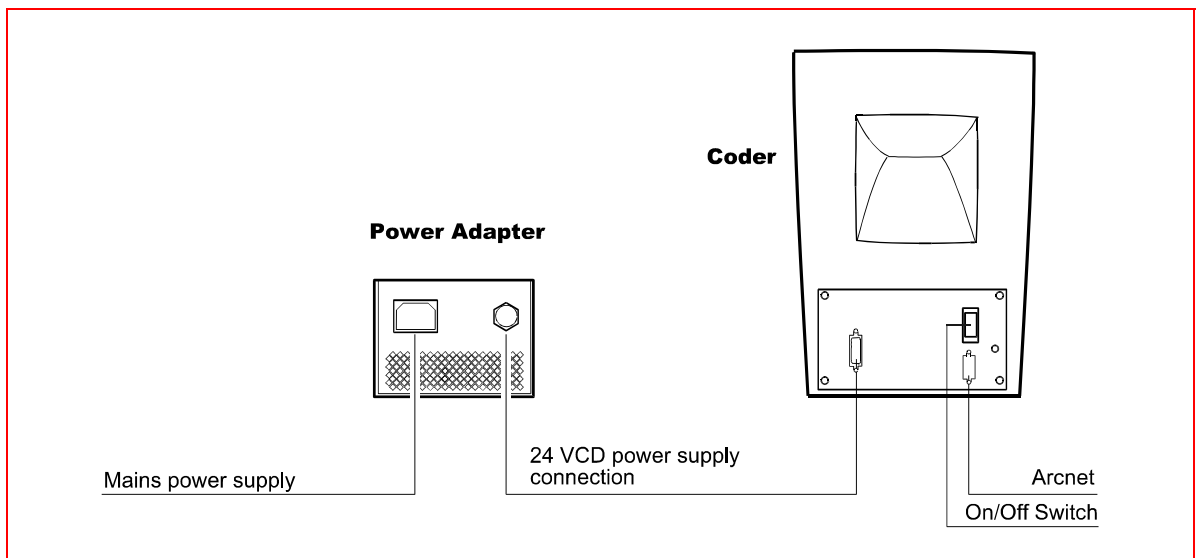
Fig. 1: Connections Coder MC BASIC 400
