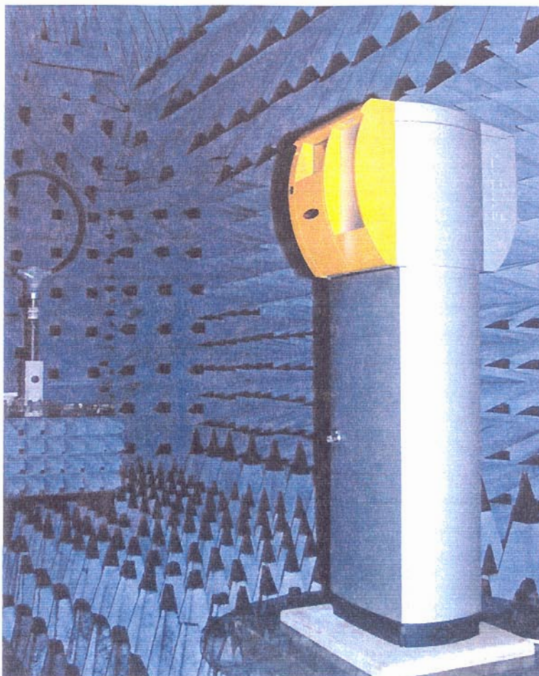
Photo No. 1, Park Column AS 450 SA00-BLL in the full anechoic chamber.
