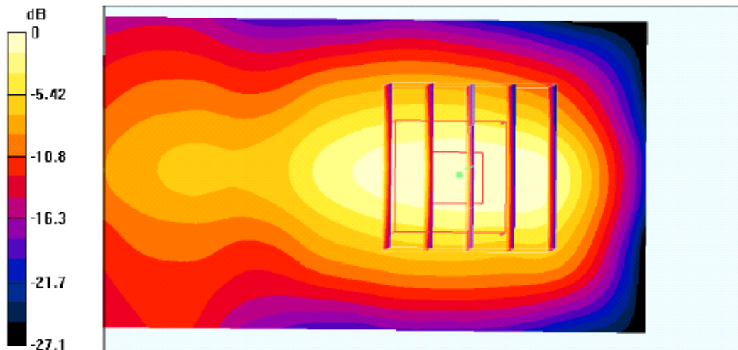
0 dB = 0.598mW/g
