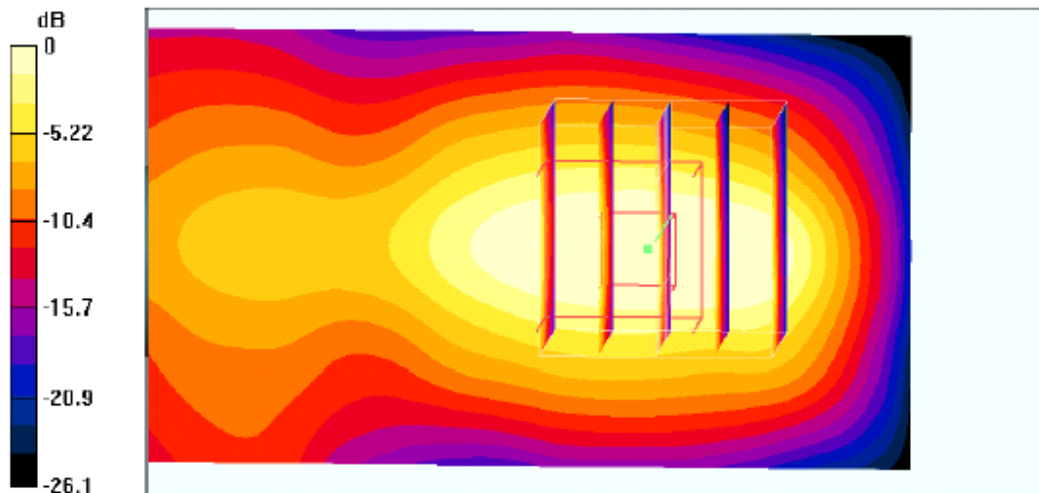
0 dB = 1.36mW/g
