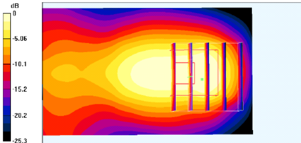
0 dB = 1.19mW/g
