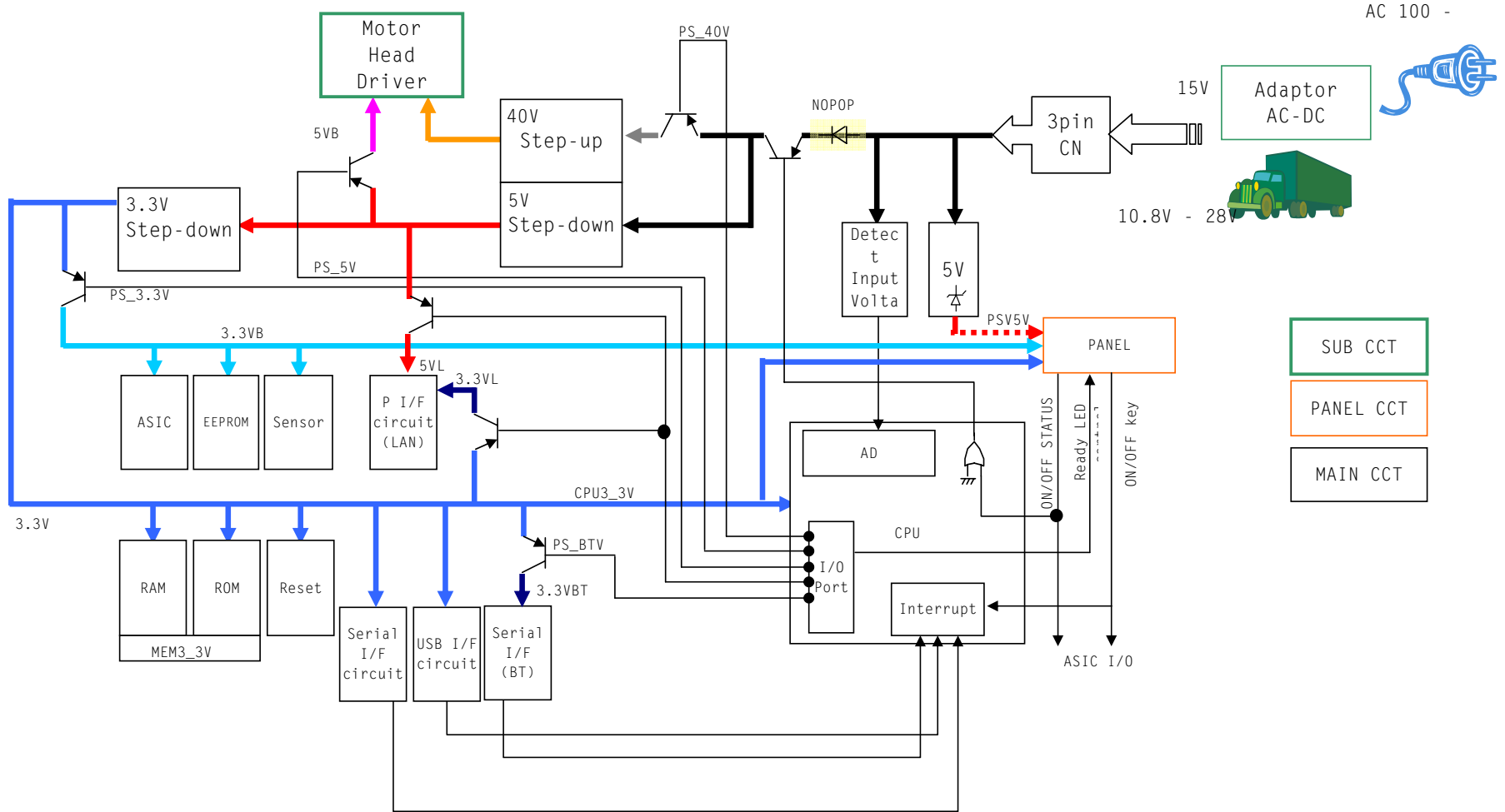
Fixed type power supply diagram
