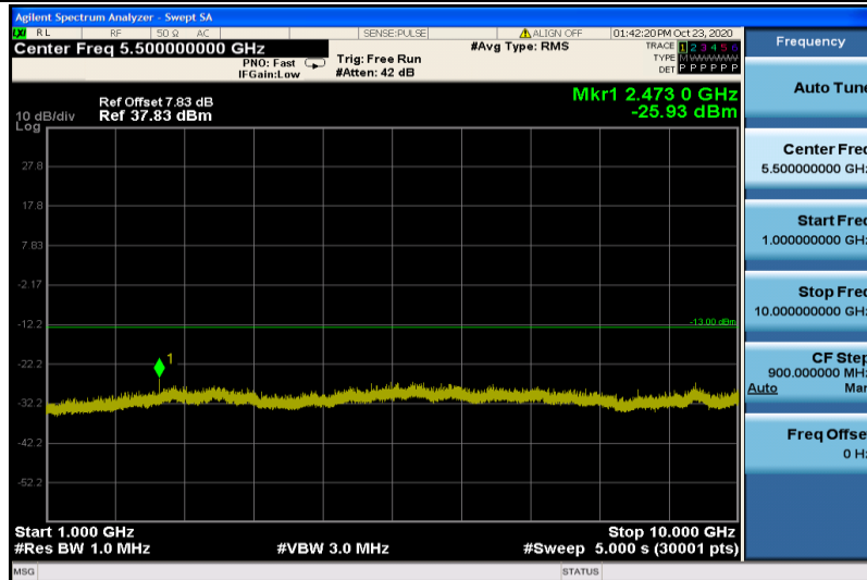
GSM850-128-1000~10000
