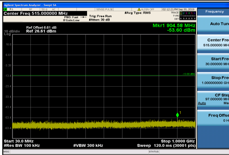
Band4-5MHz-16QAM-20175-1RB#0-30~1000MHz
