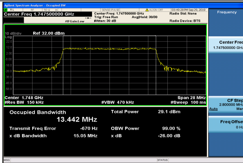
Band4-15MHz-QPSK-20325-75RB#0-13.442
