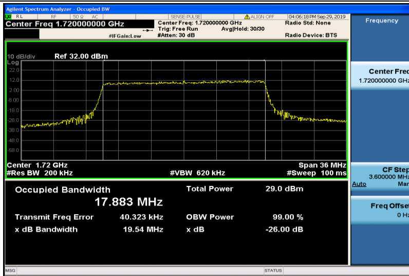
Band4-20MHz-QPSK-20050-100RB#0-17.883
