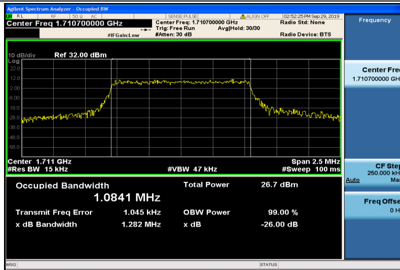
Band4-1.4MHz-16QAM-19957-6RB#0-1.0841
