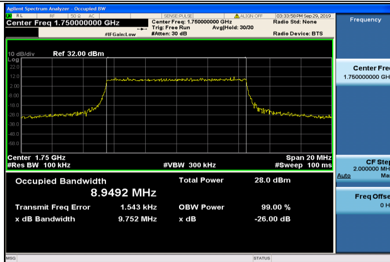
Band4-10MHz-16QAM-20350-50RB#0-8.9492
