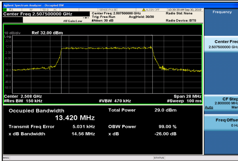
Band7-15MHz-16QAM-20825-75RB#0-13.420
