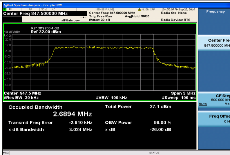
Band5-3MHz-16QAM-20635-15RB#0-2.6894
