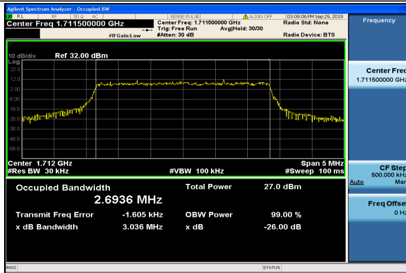
Band4-3MHz-16QAM-19965-15RB#0-2.6936
