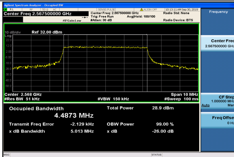
Band7-5MHz-16QAM-21425-25RB#0-4.4873
