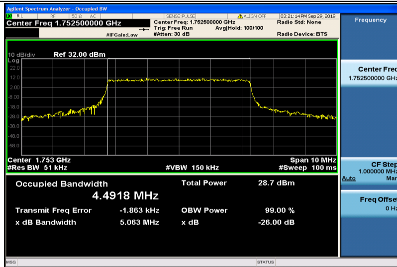
Band4-5MHz-QPSK-20375-25RB#0-4.4918
