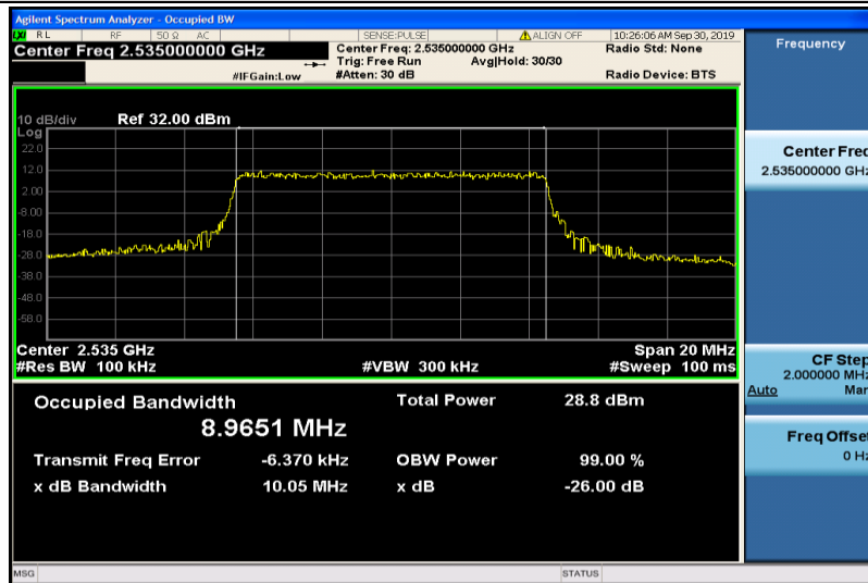
Band7-10MHz-16QAM-21100-50RB#0-8.9651
