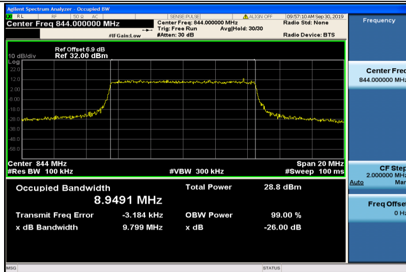
Band5-10MHz-16QAM-20600-50RB#0-8.9491
