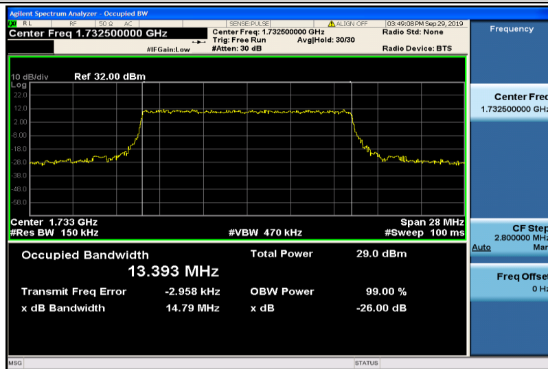
Band4-15MHz-QPSK-20175-75RB#0-13.393
