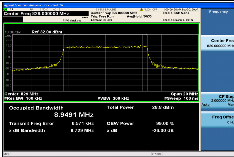
Band5-10MHz-16QAM-20450-50RB#0-8.9491
