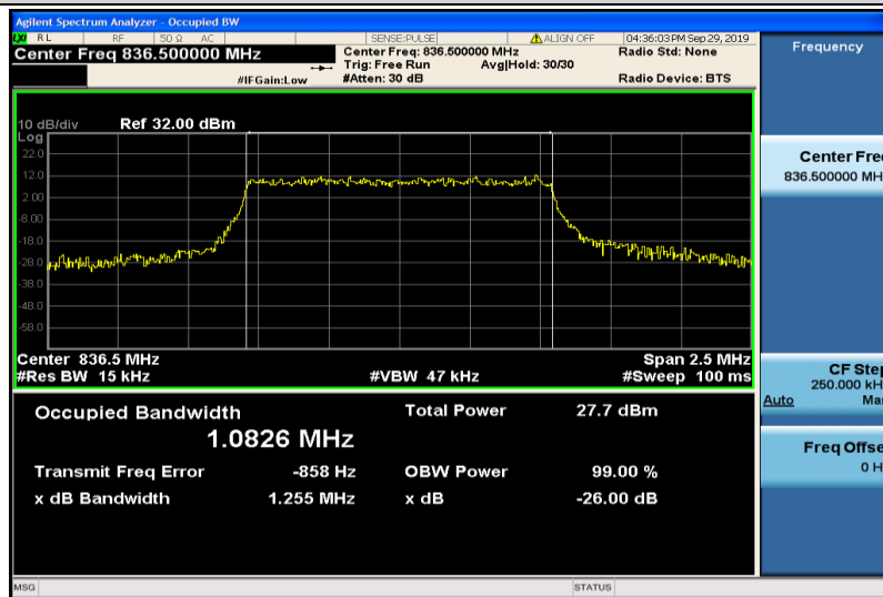
Band5-1.4MHz-QPSK-20525-6RB#0-1.0826
