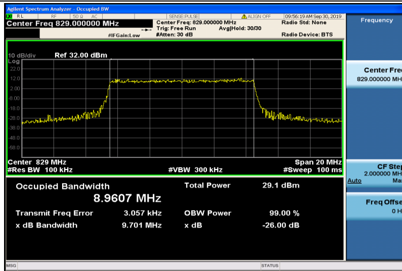
Band5-10MHz-QPSK-20450-50RB#0-8.9607
