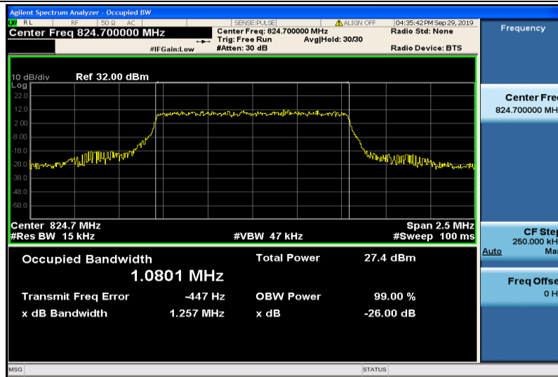
Band5-1.4MHz-QPSK-20407-6RB#0-1.0801
