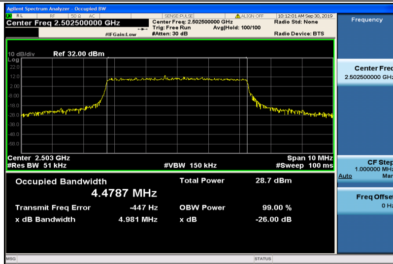
Band7-5MHz-16QAM-20775-25RB#0-4.4787
