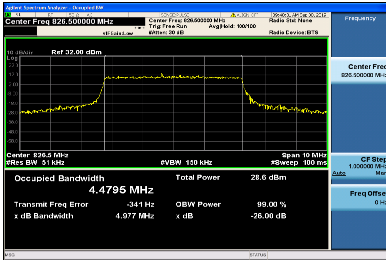
Band5-5MHz-16QAM-20425-25RB#0-4.4795
