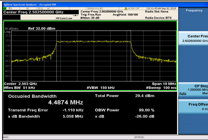
Band7-5MHz-QPSK-20775-25RB#0-4.4874
