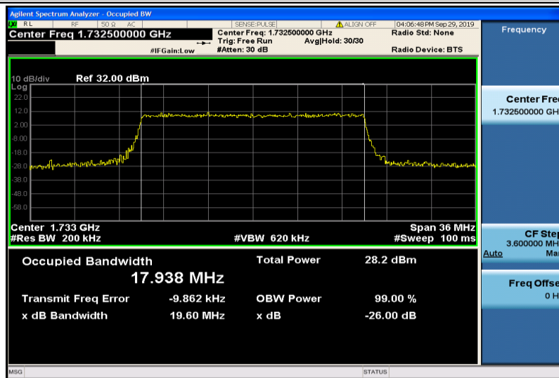
Band4-20MHz-16QAM-20175-100RB#0-17.938
