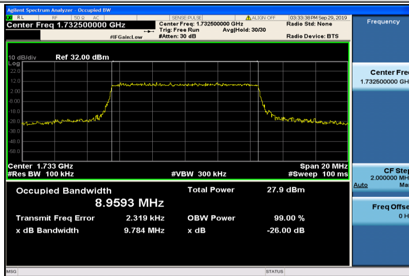
Band4-10MHz-16QAM-20175-50RB#0-8.9593
