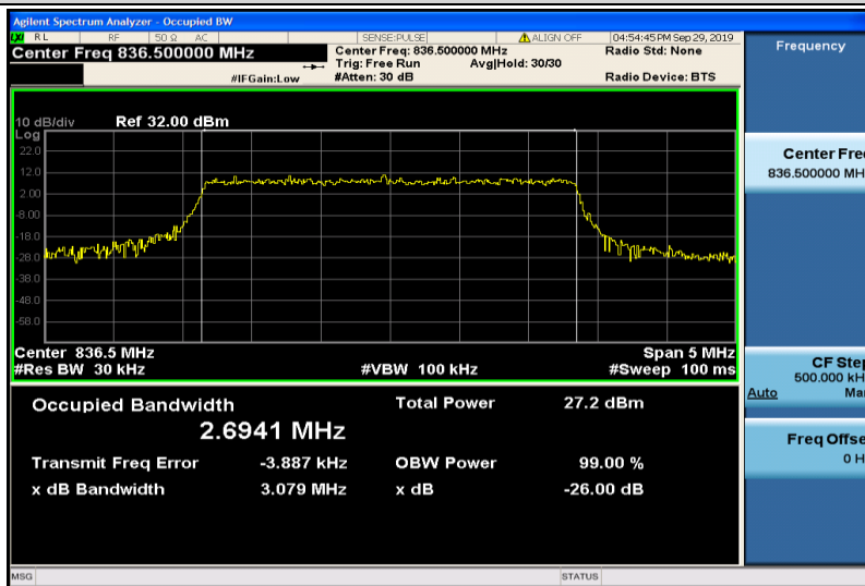
Band5-3MHz-16QAM-20525-15RB#0-2.6941
