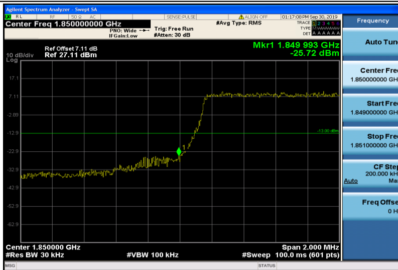
Band2-1.4MHz-QPSK-18607-6RB#0
