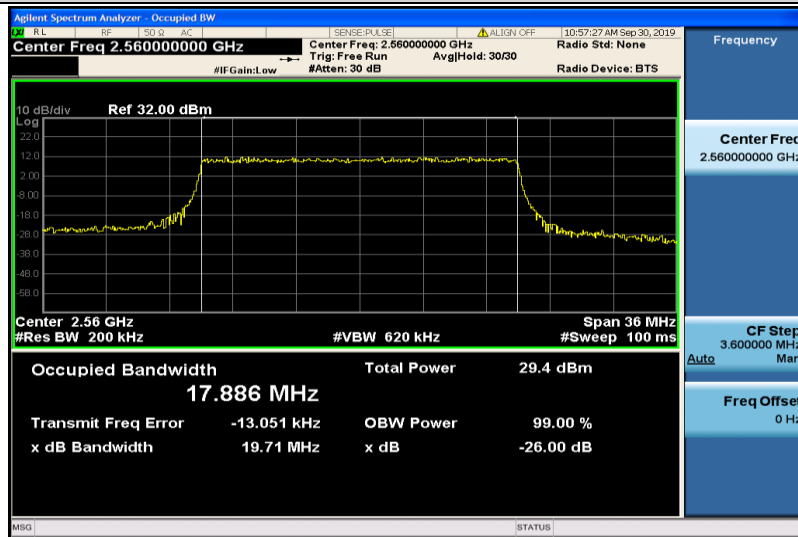
Band7-20MHz-16QAM-21350-100RB#0-17.886
