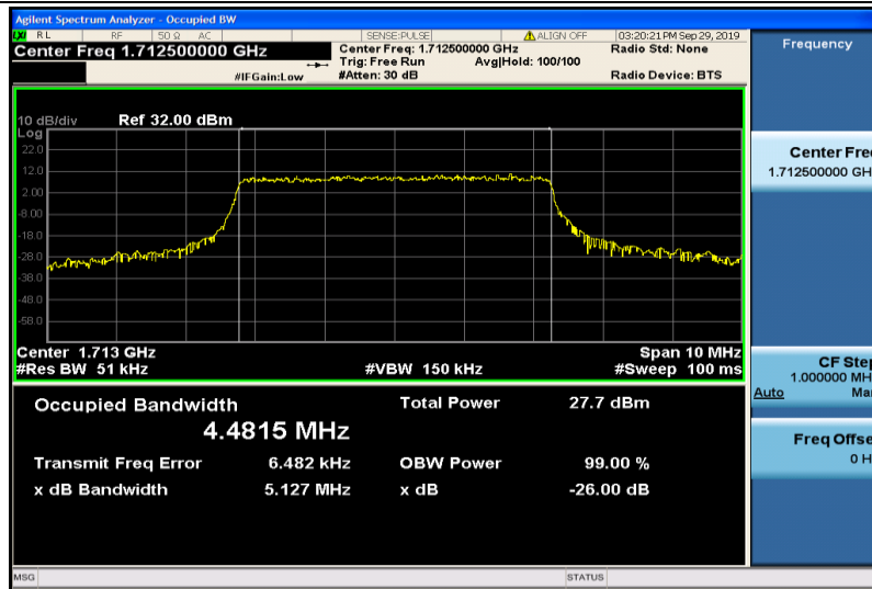
Band4-5MHz-16QAM-19975-25RB#0-4.4815
