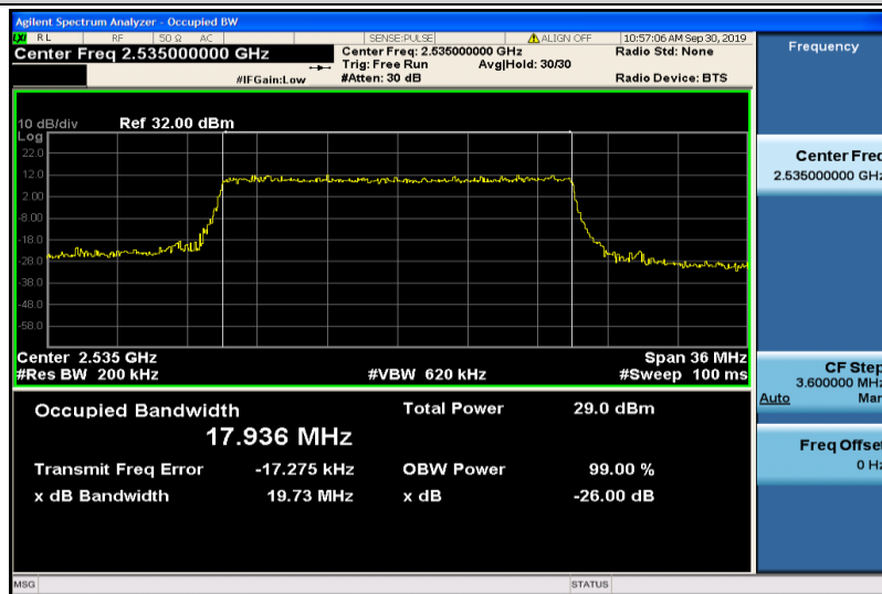
Band7-20MHz-16QAM-21100-100RB#0-17.936
