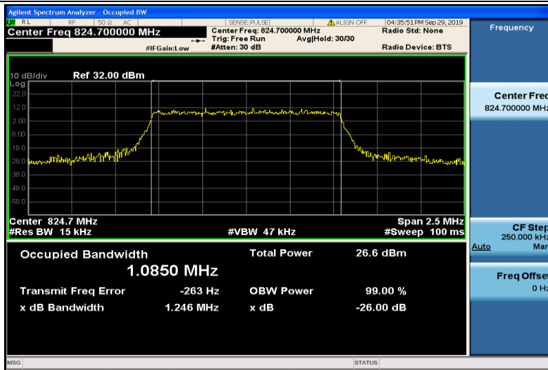
Band5-1.4MHz-16QAM-20407-6RB#0-1.0850
