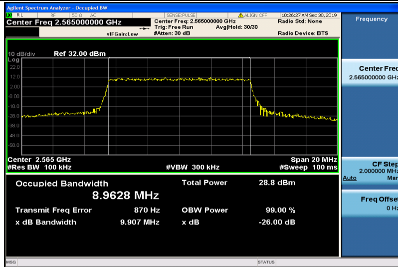
Band7-10MHz-16QAM-21400-50RB#0-8.9628
