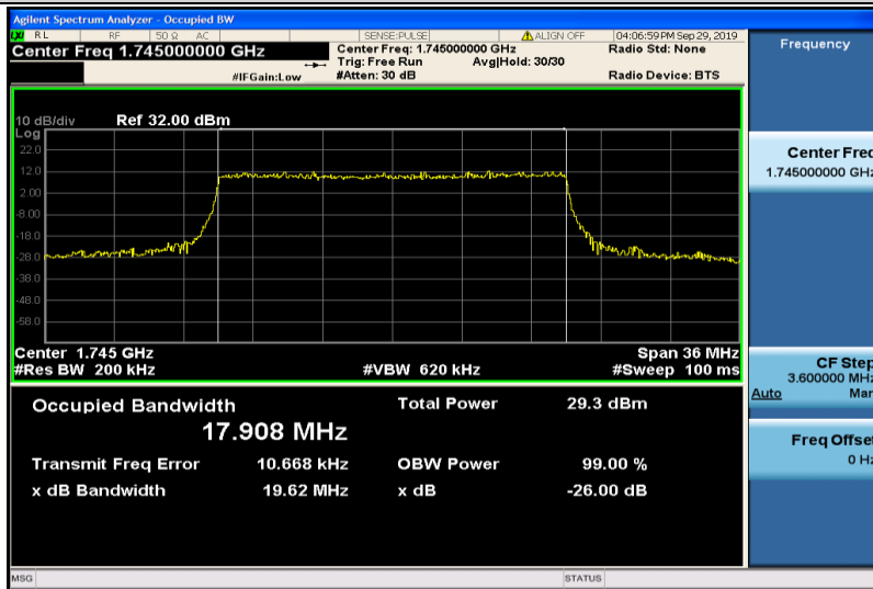
Band4-20MHz-QPSK-20300-100RB#0-17.908
