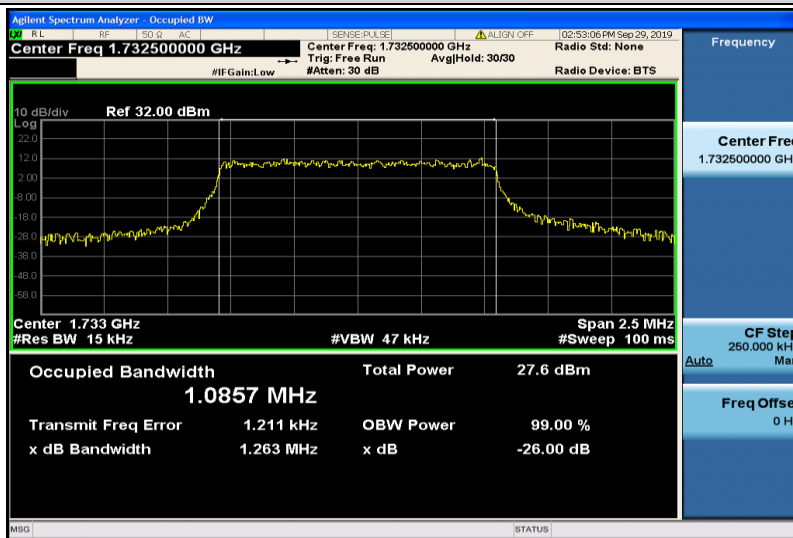
Band4-1.4MHz-QPSK-20175-6RB#0-1.0857
