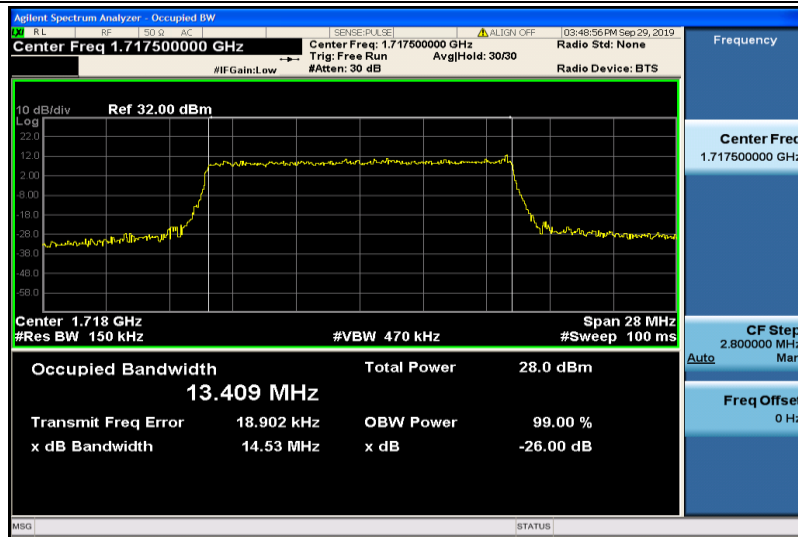
Band4-15MHz-16QAM-20025-75RB#0-13.409
