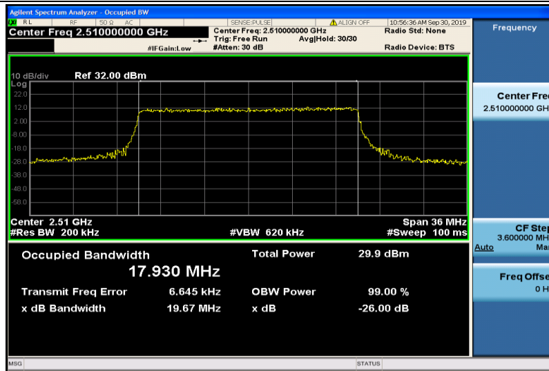
Band7-20MHz-QPSK-20850-100RB#0-17.930
