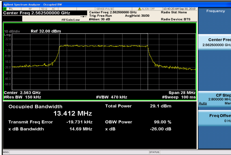
Band7-15MHz-16QAM-21375-75RB#0-13.412
