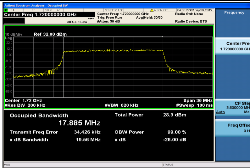
Band4-20MHz-16QAM-20050-100RB#0-17.885
