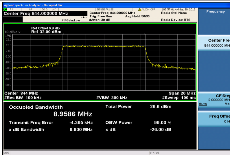
Band5-10MHz-QPSK-20600-50RB#0-8.9586
