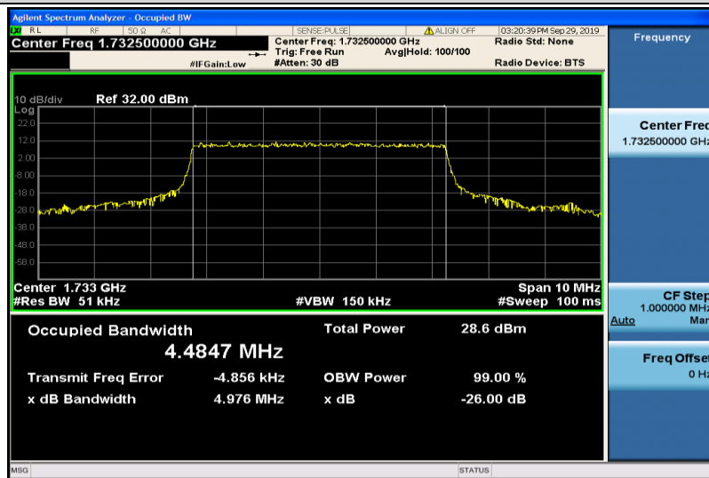
Band4-5MHz-QPSK-1732500000-4.4847
