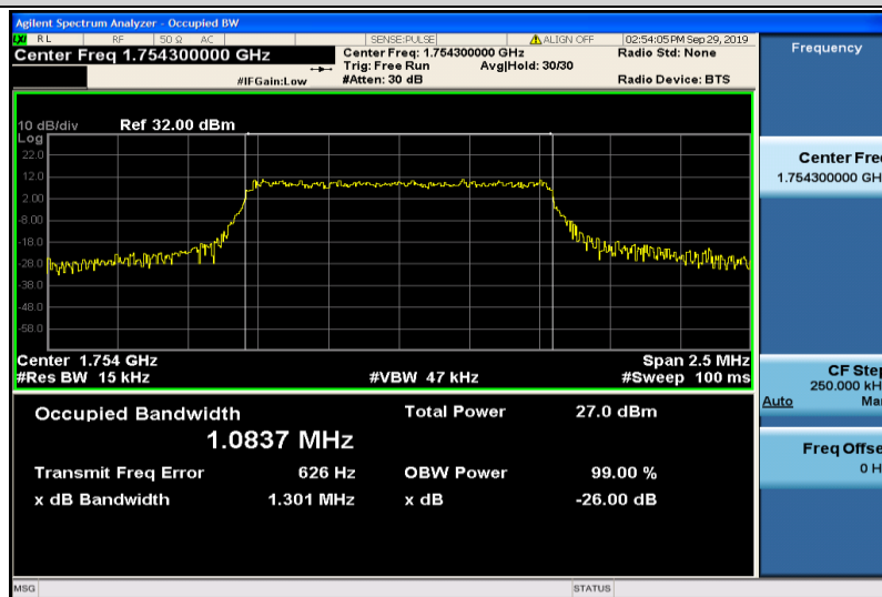
Band4-1.4MHz-16QAM-20393-6RB#0-1.0837
