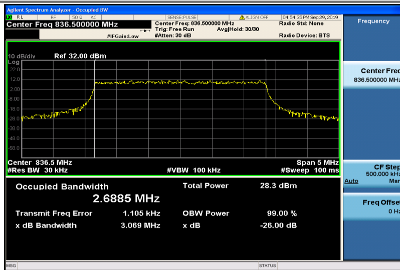
Band5-3MHz-QPSK-20525-15RB#0-2.6885
