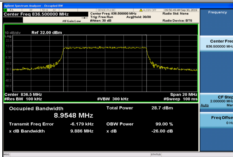
Band5-10MHz-16QAM-20525-50RB#0-8.9548
