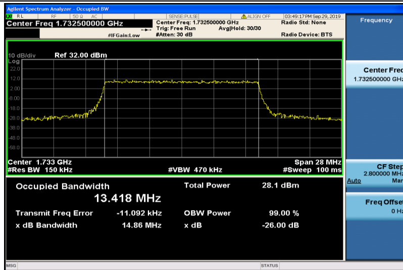
Band4-15MHz-16QAM-20175-75RB#0-13.418
