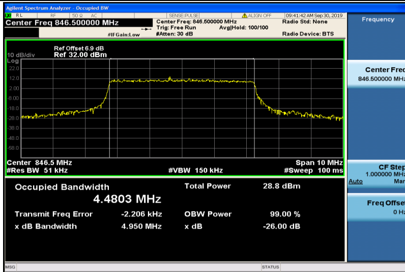
Band5-5MHz-16QAM-20625-25RB#0-4.4803
