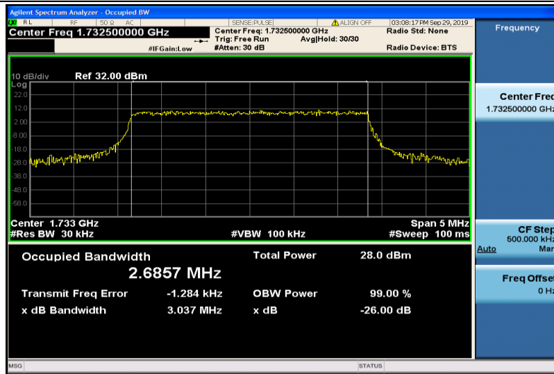
Band4-3MHz-QPSK-20175-15RB#0-2.6857
