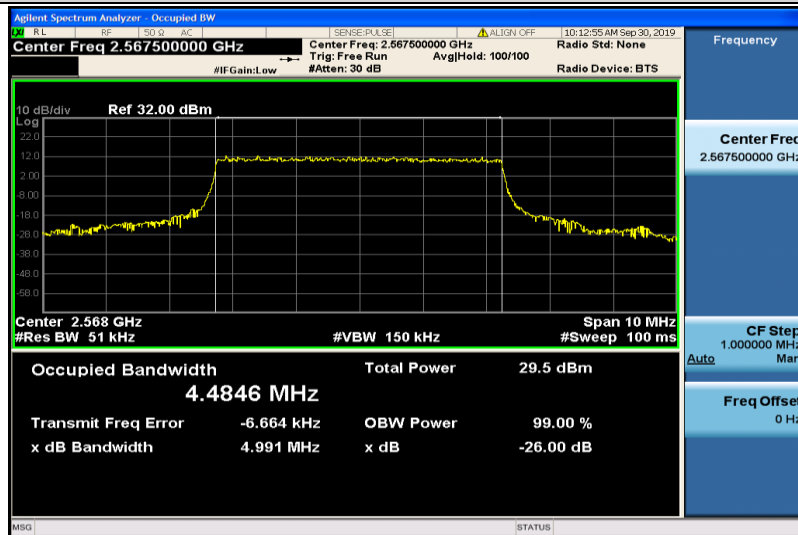
Band7-5MHz-QPSK-21425-25RB#0-4.4846
