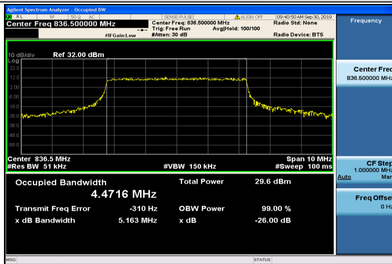
Band5-5MHz-QPSK-20525-25RB#0-4.4716
