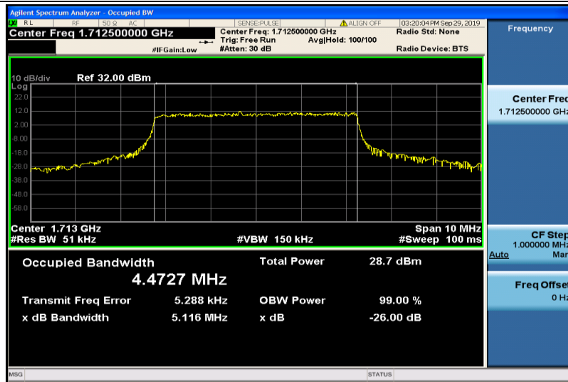
Band4-5MHz-QPSK-19975-25RB#0-4.4727
