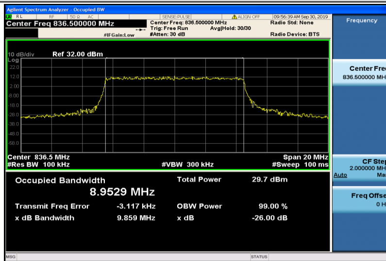
Band5-10MHz-QPSK-20525-50RB#0-8.9529
