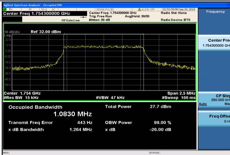
Band4-1.4MHz-QPSK-20393-6RB#0-1.0830
