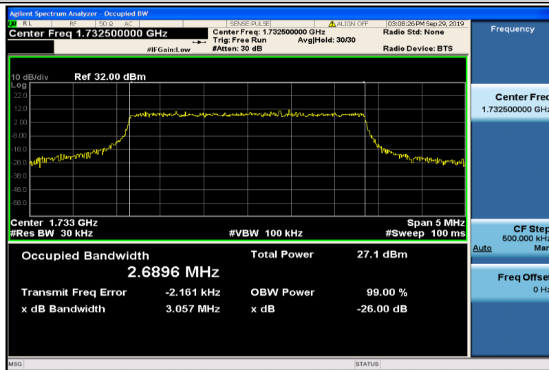
Band4-3MHz-16QAM-20175-15RB#0-2.6896
