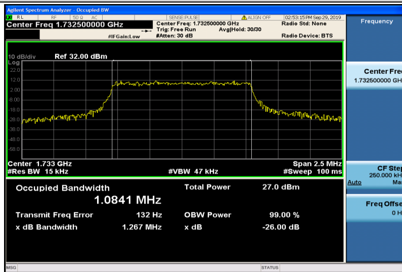
Band4-1.4MHz-16QAM-17325-6RB#0-1.0841
