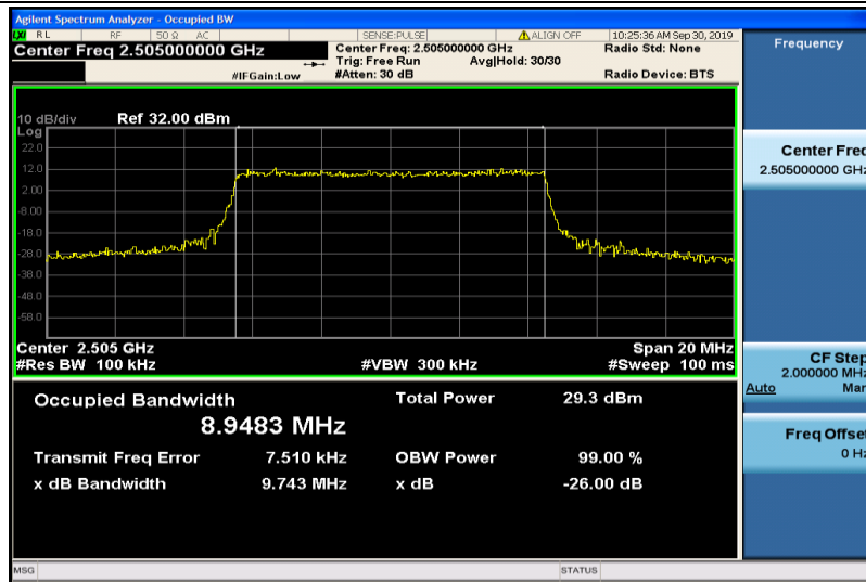
Band7-10MHz-QPSK-20800-50RB#0-8.9483
