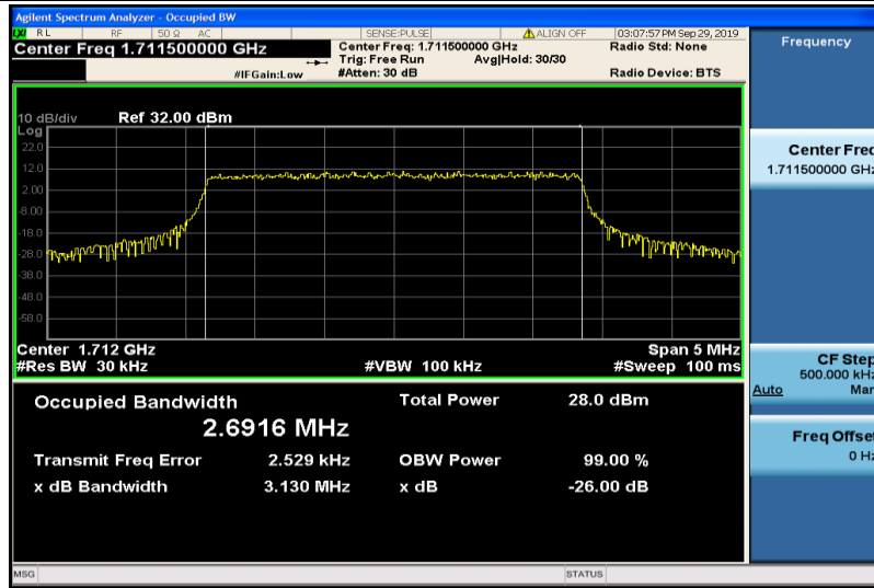
Band4-3MHz-QPSK-19965-15RB#0-2.6916
