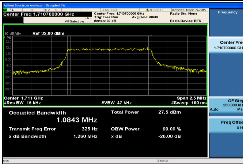
Band4-1.4MHz-QPSK-19957-6RB#0-1.0843
