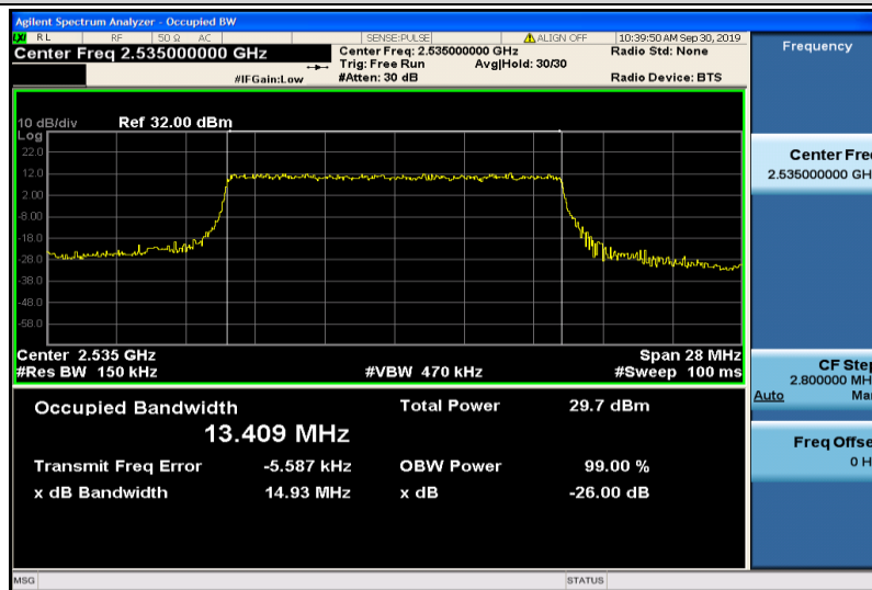
Band7-15MHz-QPSK-21100-75RB#0-13.409
