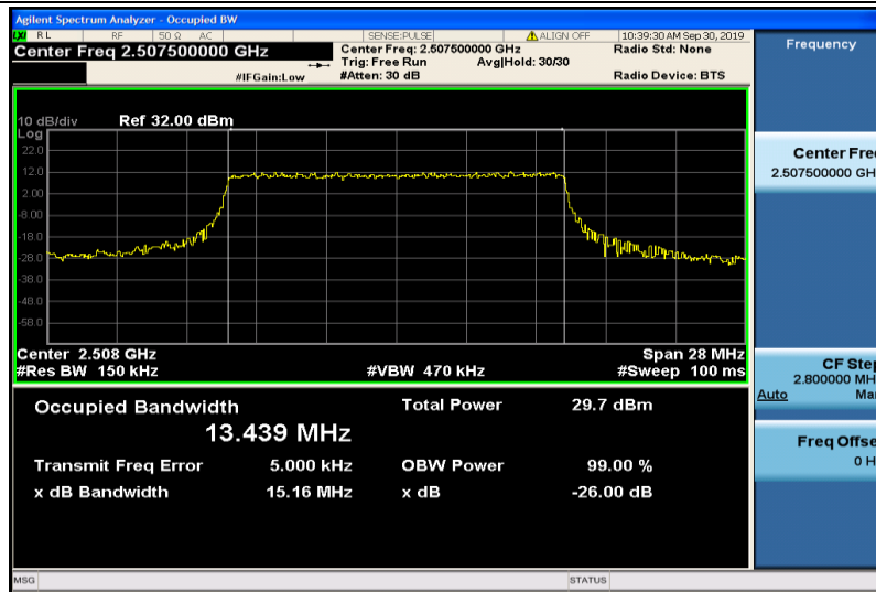
Band7-15MHz-QPSK-20825-75RB#0-13.439
