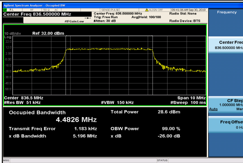
Band5-5MHz-16QAM-20525-25RB#0-4.4826
