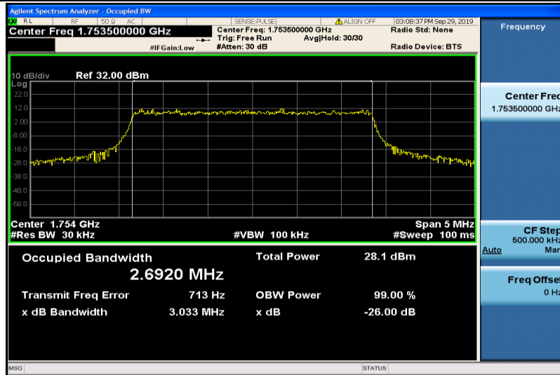
Band4-3MHz-QPSK-20385-15RB#0-2.6920
