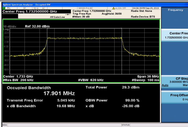
Band4-20MHz-QPSK-20175-100RB#0-17.901
