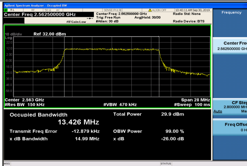
Band7-15MHz-QPSK-21375-75RB#0-13.426
