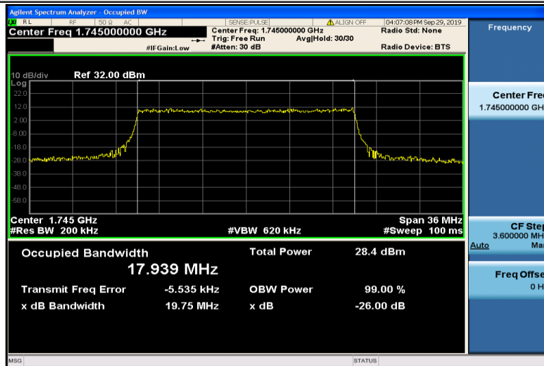
Band4-20MHz-16QAM-20300-100RB#0-17.939
