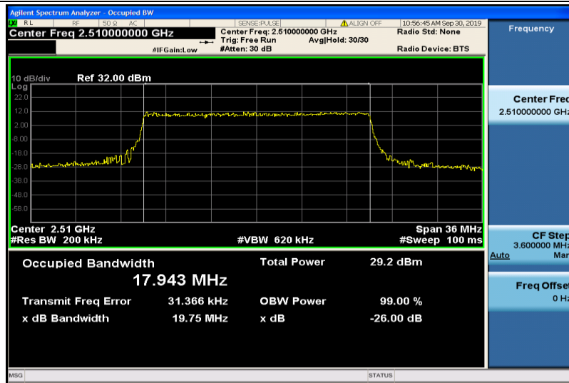
Band7-20MHz-16QAM-20850-100RB#0-17.943
