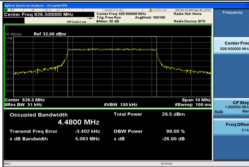
Band5-5MHz-QPSK-20425-25RB#0-4.4800
