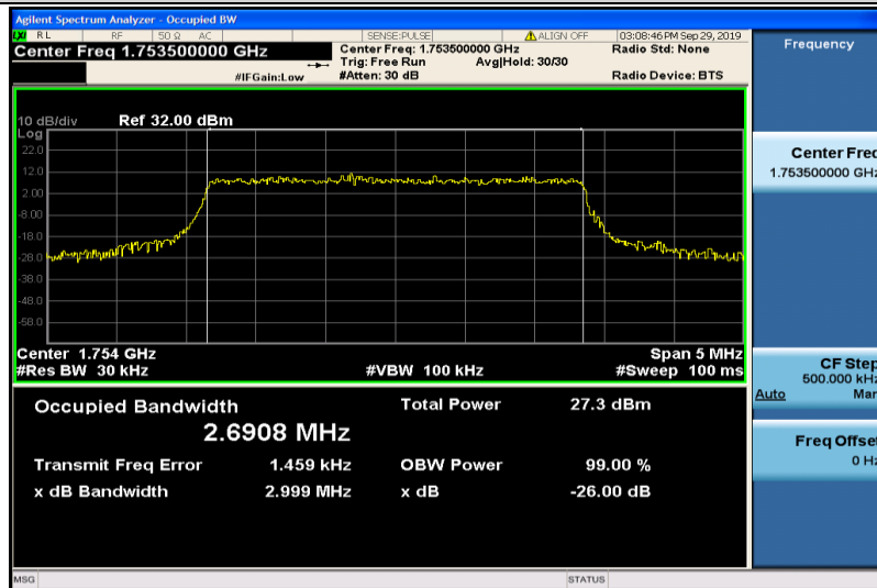
Band4-3MHz-16QAM-20385-15RB#0-2.6908
