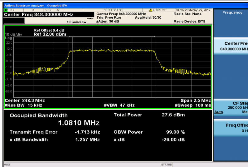
Band5-1.4MHz-QPSK-20643-6RB#0-1.0810
