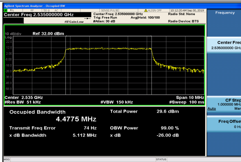
Band7-5MHz-QPSK-21100-25RB#0-4.4775
