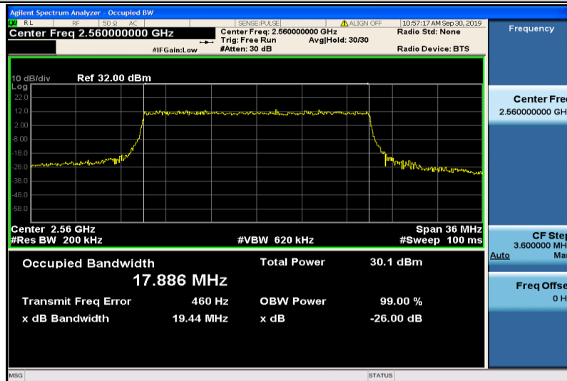
Band7-20MHz-QPSK-21350-100RB#0-17.886
