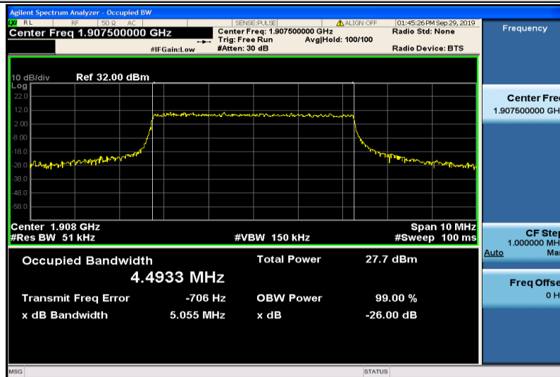
Band2-5MHz-16QAM-19175-25RB#0-4.4933
