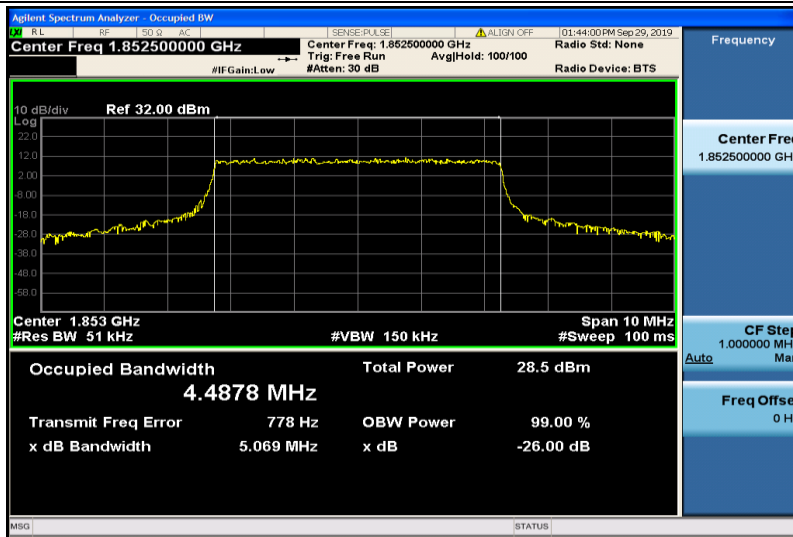
Band2-5MHz-QPSK-18625-25RB#0-4.4878
