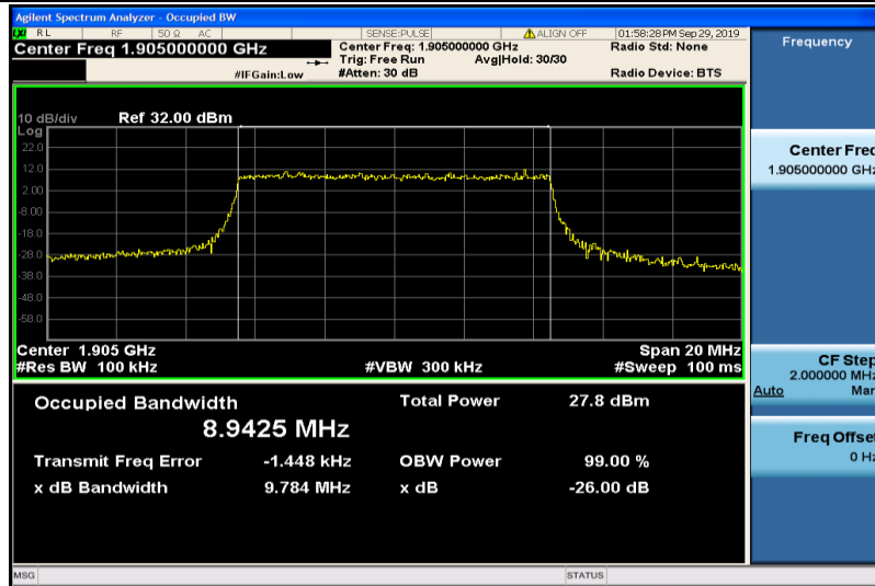
Band2-10MHz-16QAM-19150-50RB#0-8.9425
