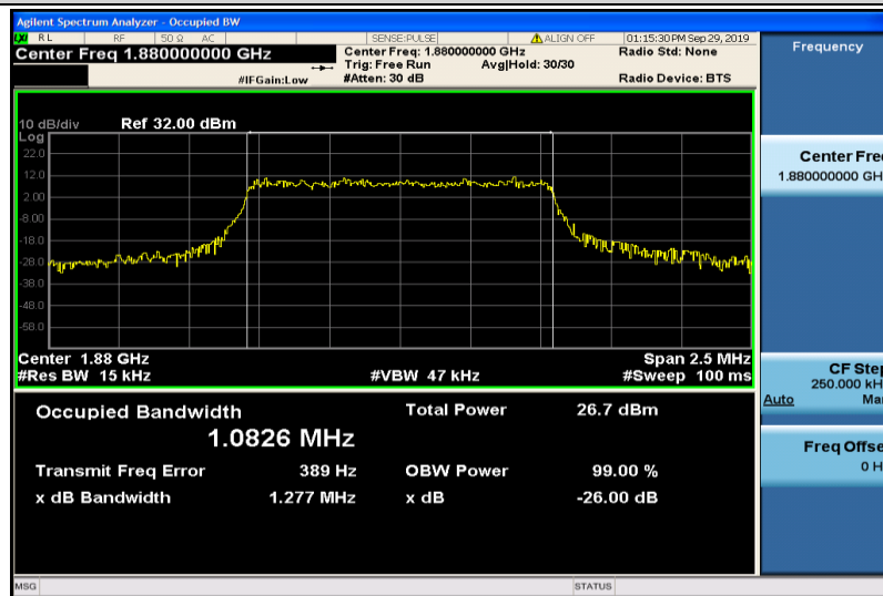
Band2-1.4MHz-16QAM-18900-6RB#0-1.0826
