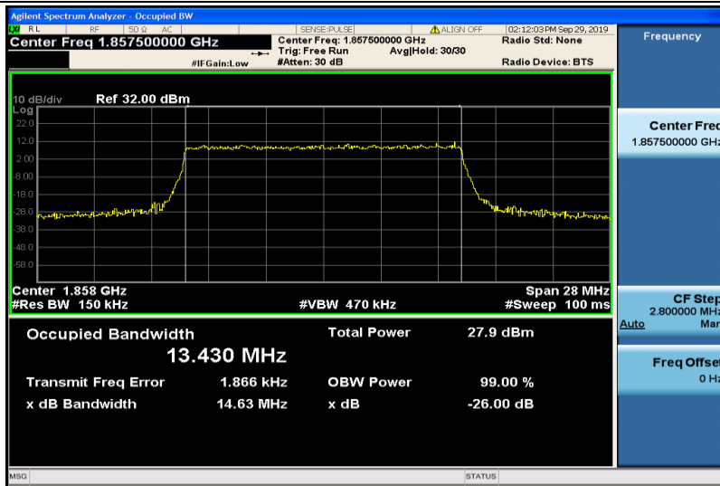
Band2-15MHz-16QAM-18675-75RB#0-13.430
