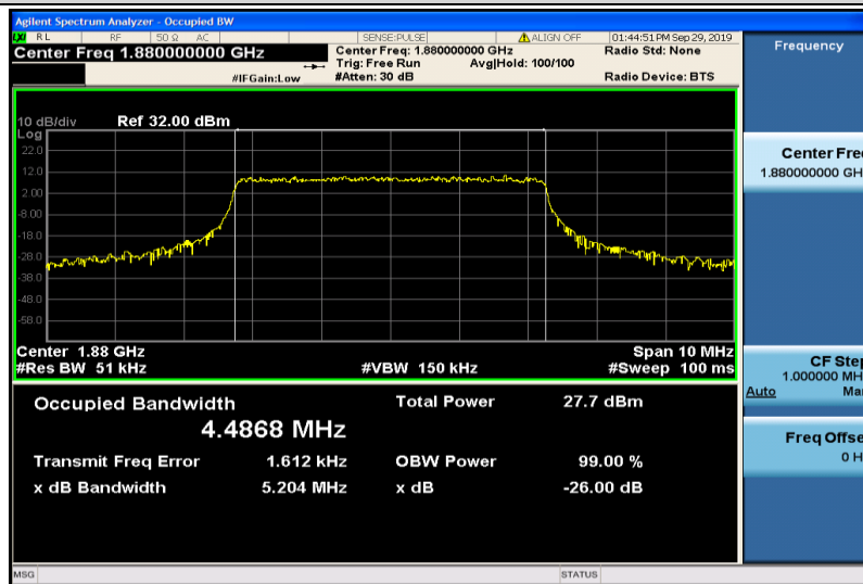
Band2-5MHz-16QAM-18900-25RB#0-4.4868
