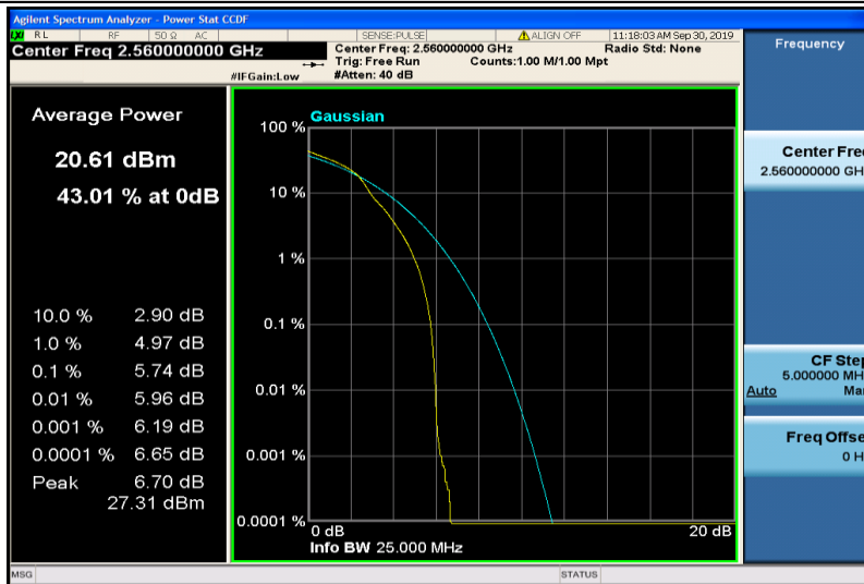
Band7-20MHz-16QAM-21350-1RB#0
