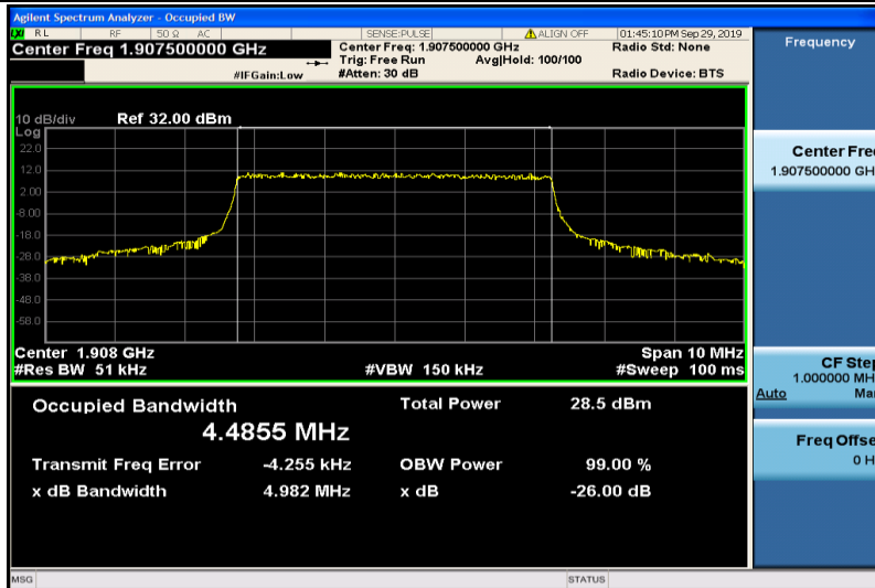
Band2-5MHz-QPSK-19175-25RB#0-4.4855
