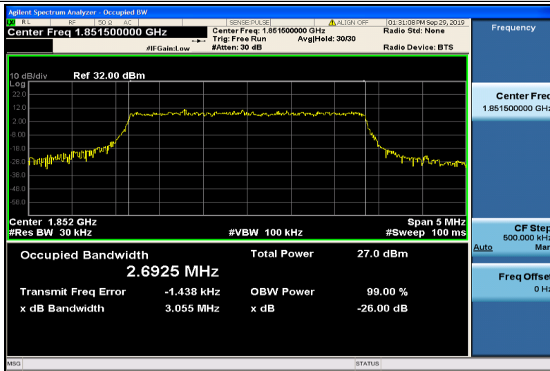
Band2-3MHz-16QAM-18615-15RB#0-2.6925
