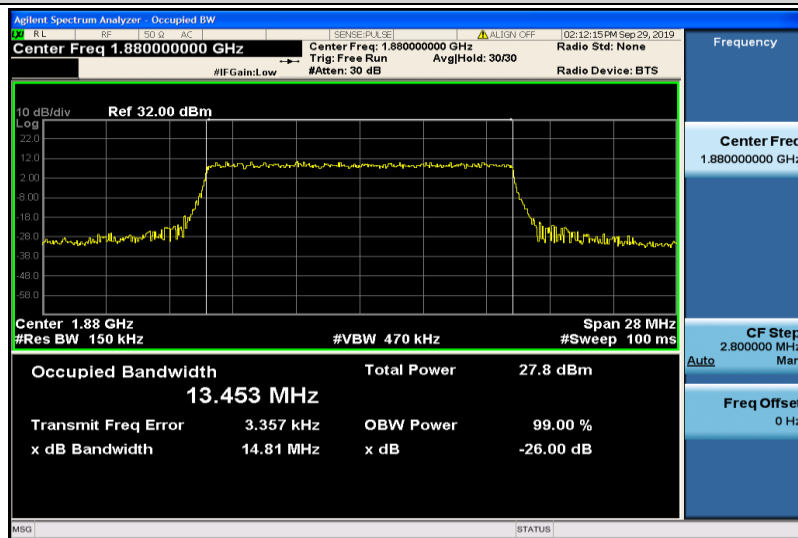
Band2-15MHz-QPSK-18900-75RB#0-13.453
