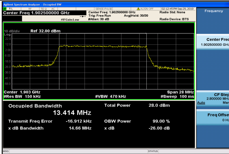
Band2-15MHz-16QAM-19125-75RB#0-13.414
