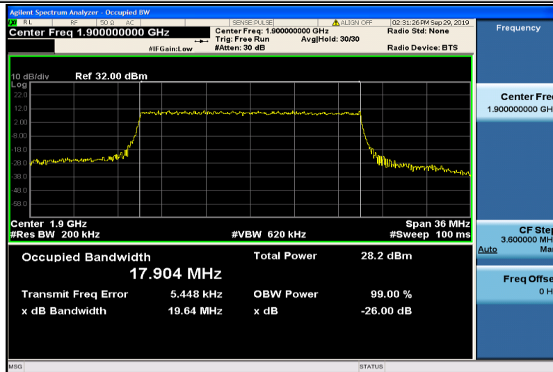
Band2-20MHz-16QAM-19100-100RB#0-17.904
