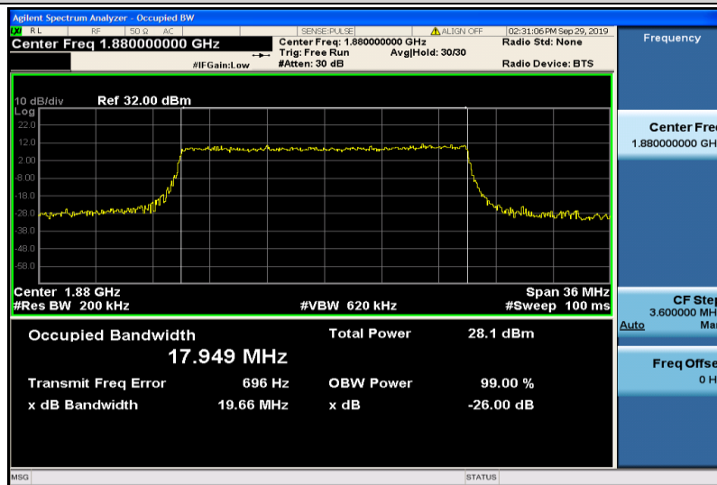
Band2-20MHz-16QAM-18900-100RB#0-17.949
