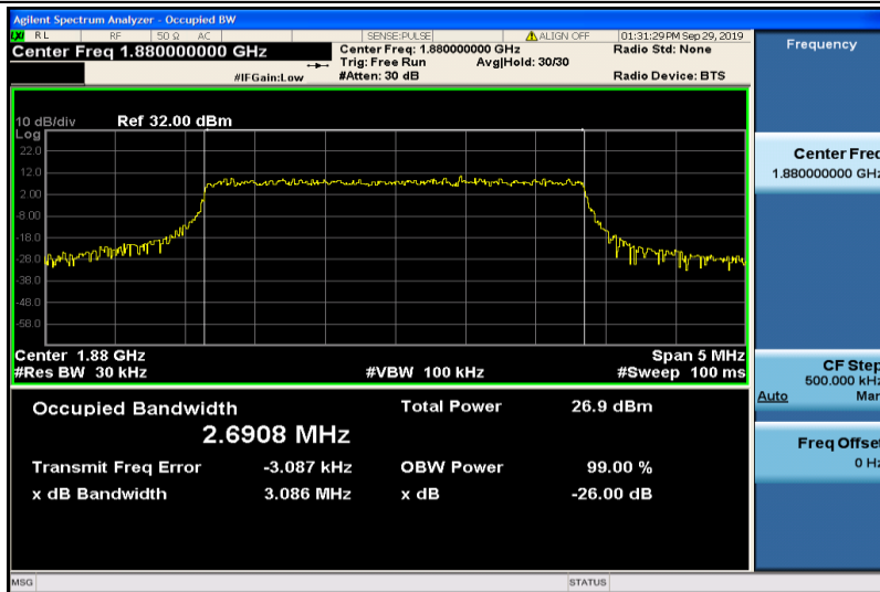
Band2-3MHz-16QAM-18900-15RB#0-2.6908
