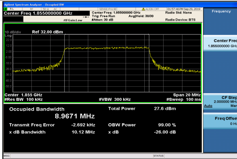
Band2-10MHz-16QAM-18650-50RB#0-8.9671
