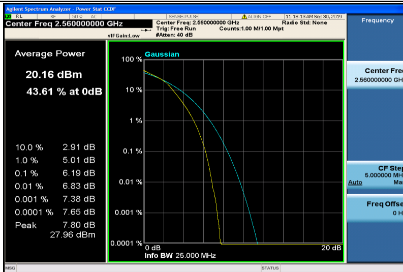
Band7-20MHz-16QAM-21350-100RB#0
