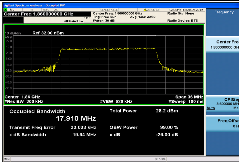
Band2-20MHz-16QAM-18700-100RB#0-17.910
