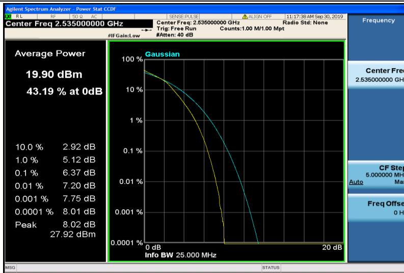
Band7-20MHz-16QAM-21100-100RB#0
