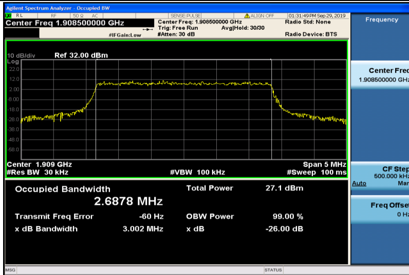
Band2-3MHz-16QAM-19185-15RB#0-2.6878
