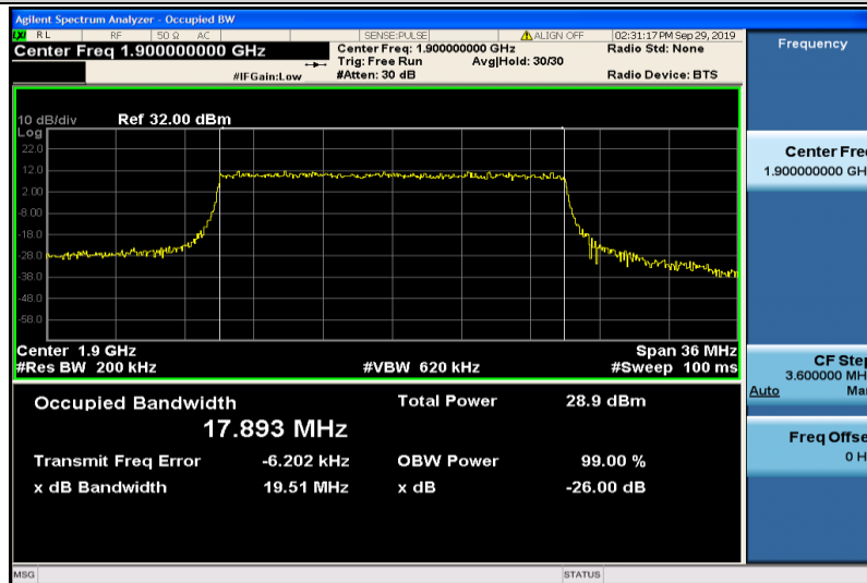
Band2-20MHz-QPSK-19100-100RB#0-17.893
