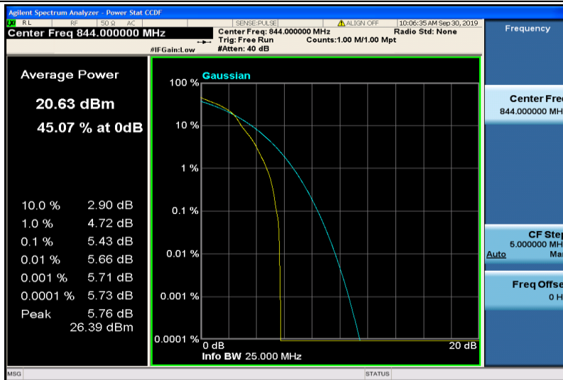
Band5-10MHz-16QAM-20600-1RB#0
