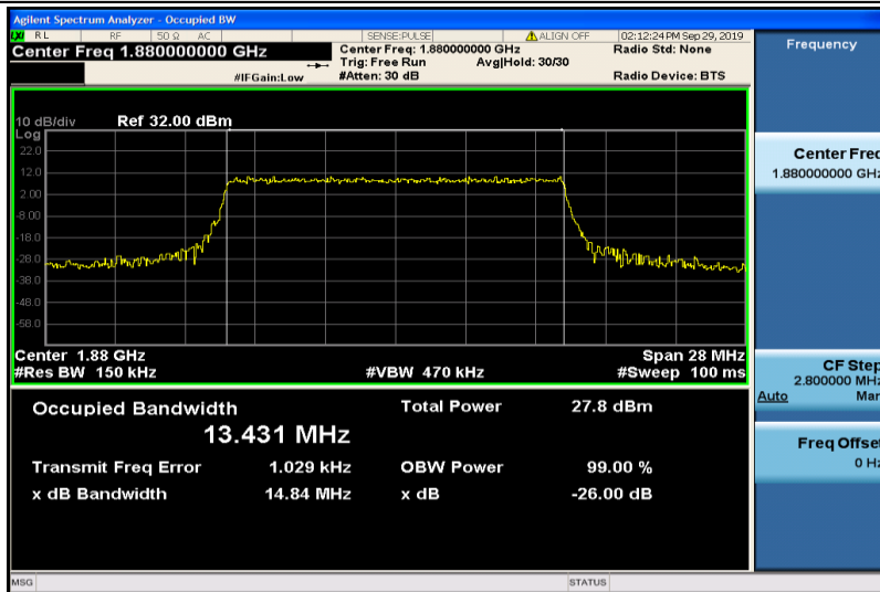
Band2-15MHz-16QAM-18900-75RB#0-13.431
