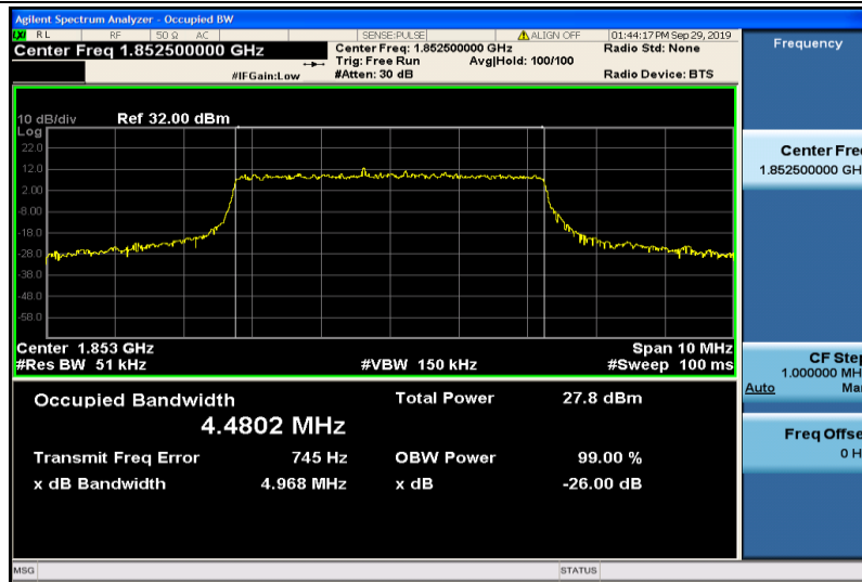
Band2-5MHz-16QAM-18625-25RB#0-4.4802
