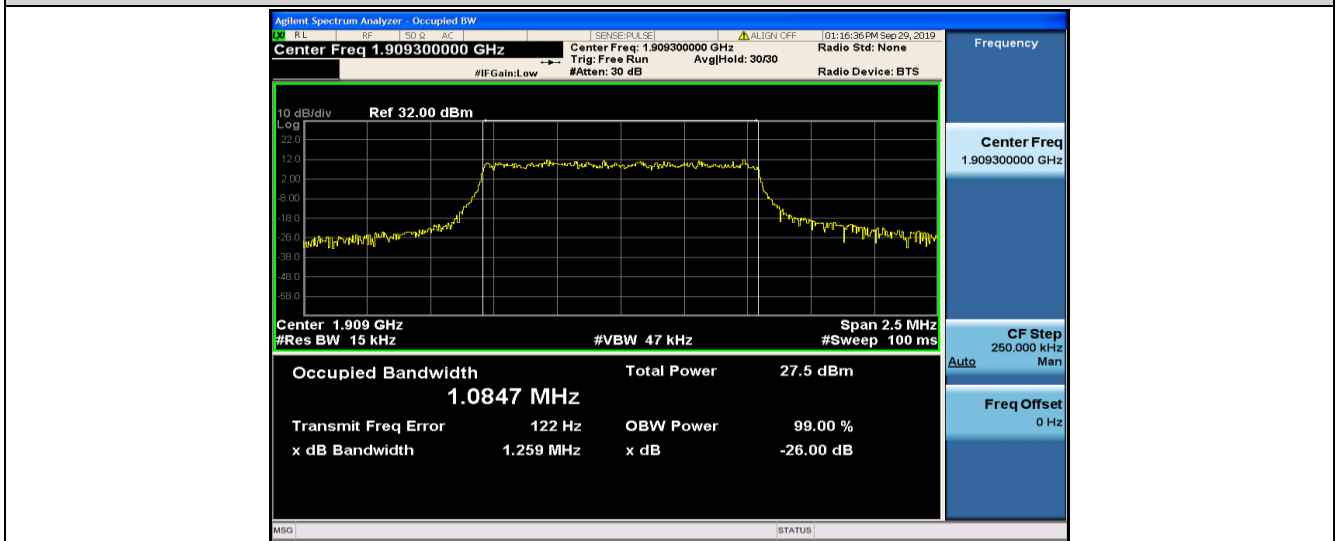
Band2-1.4MHz-QPSK-19193-6RB#0-1.0847
