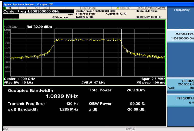
Band2-1.4MHz-16QAM-19193-6RB#0-1.0829
