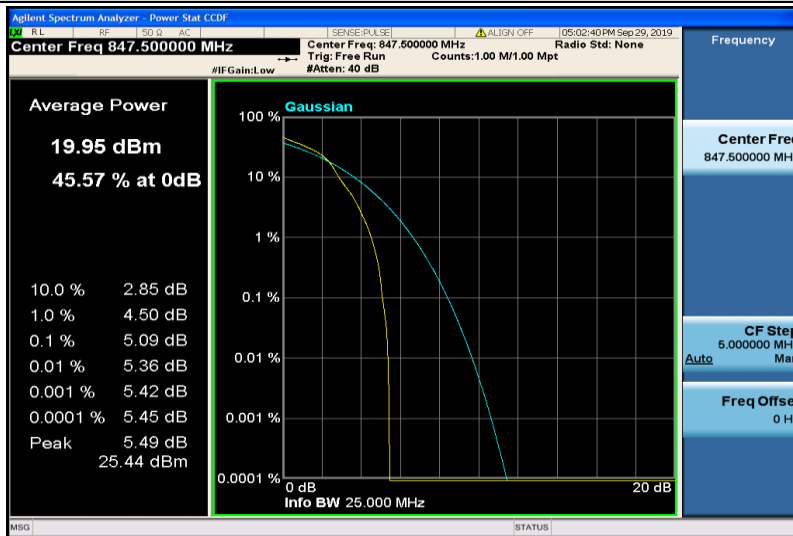
Band5-3MHz-16QAM-20635-1RB#0
