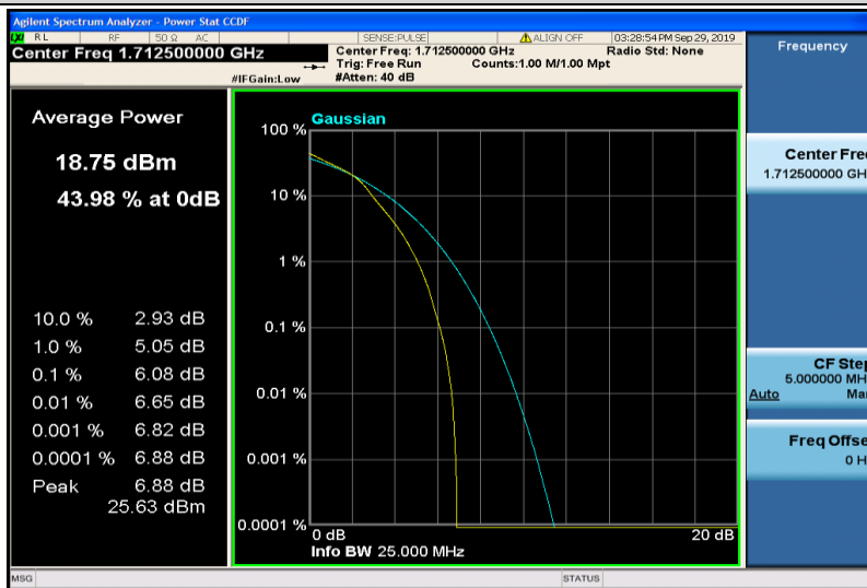
Band4-5MHz-16QAM-19975-25RB#0
