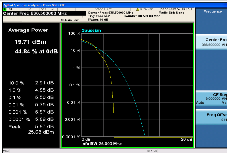
Band5-3MHz-16QAM-20525-1RB#0
