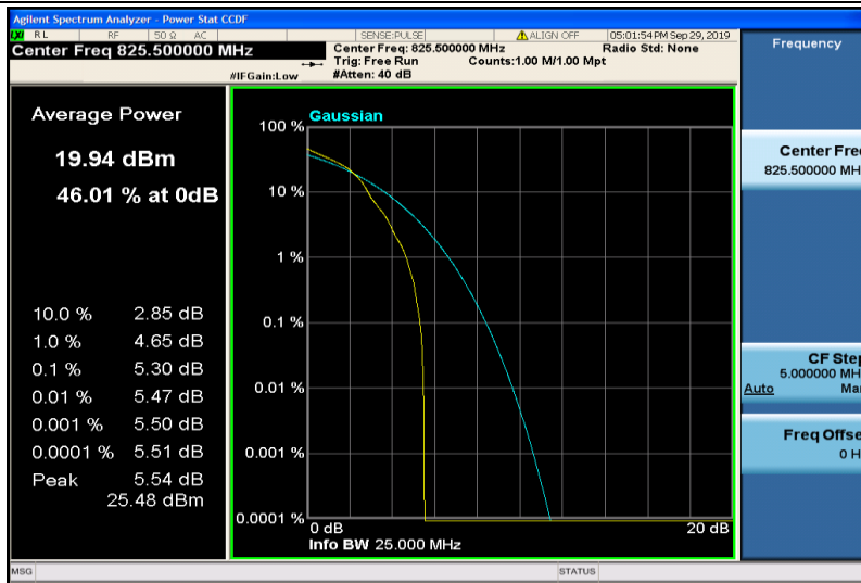
Band5-3MHz-16QAM-20415-1RB#0
