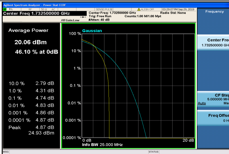
Band4-5MHz-16QAM-20175-1RB#0
