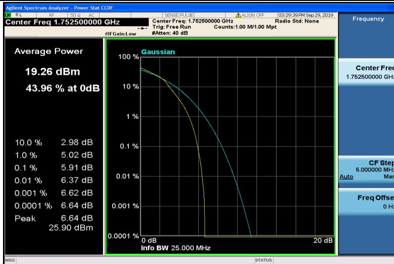
Band4-5MHz-16QAM-20375-25RB#0
