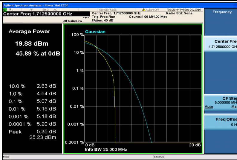
Band4-5MHz-16QAM-19975-1RB#0
