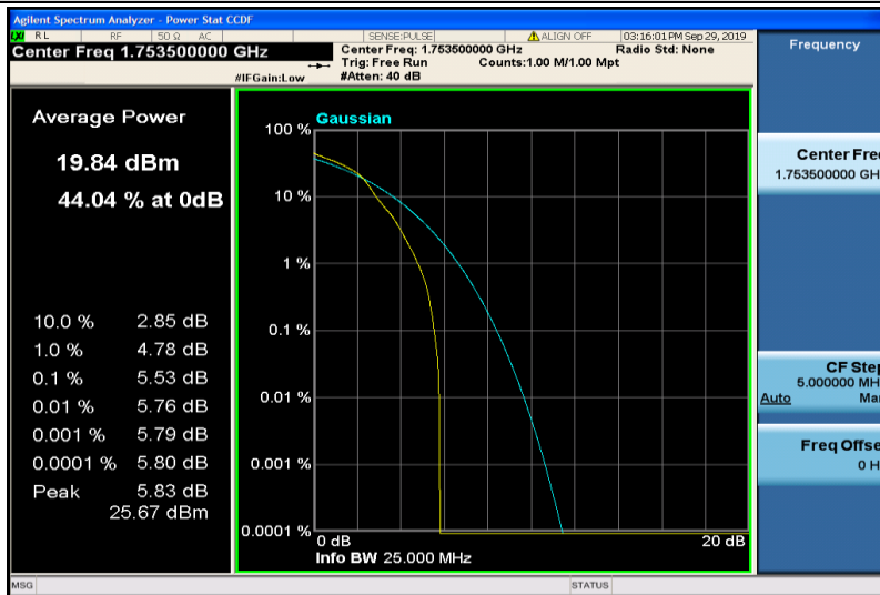
Band4-3MHz-16QAM-20385-1RB#0
