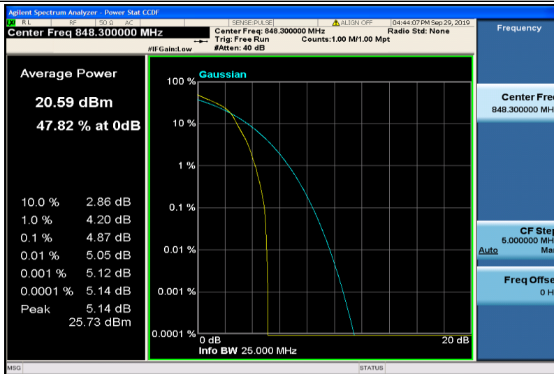
Band5-1.4MHz-16QAM-20643-1RB#0
