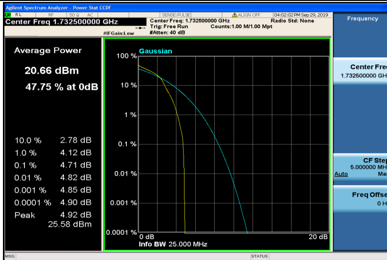
Band4-15MHz-16QAM-20175-1RB#0
