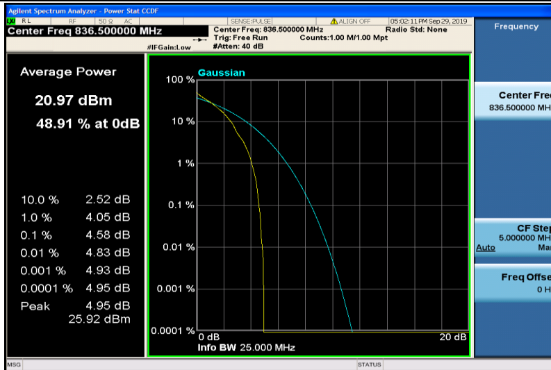
Band5-3MHz-QPSK-20525-1RB#0
