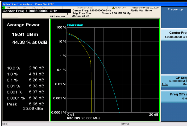
Band2-3MHz-16QAM-19185-1RB#0
