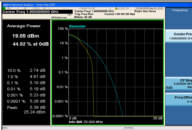
Band2-10MHz-16QAM-19150-1RB#0
