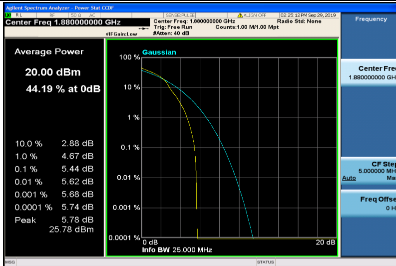
Band2-15MHz-16QAM-18900-1RB#0
