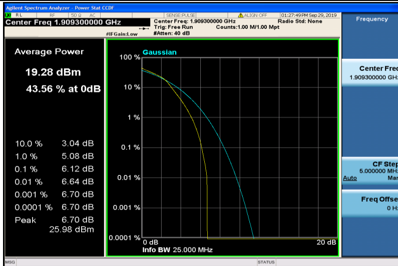
Band2-1.4MHz-16QAM-1913-6RB#0
