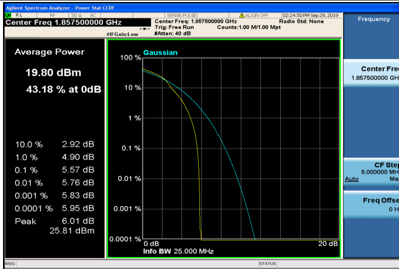
Band2-15MHz-16QAM-18675-1RB#0
