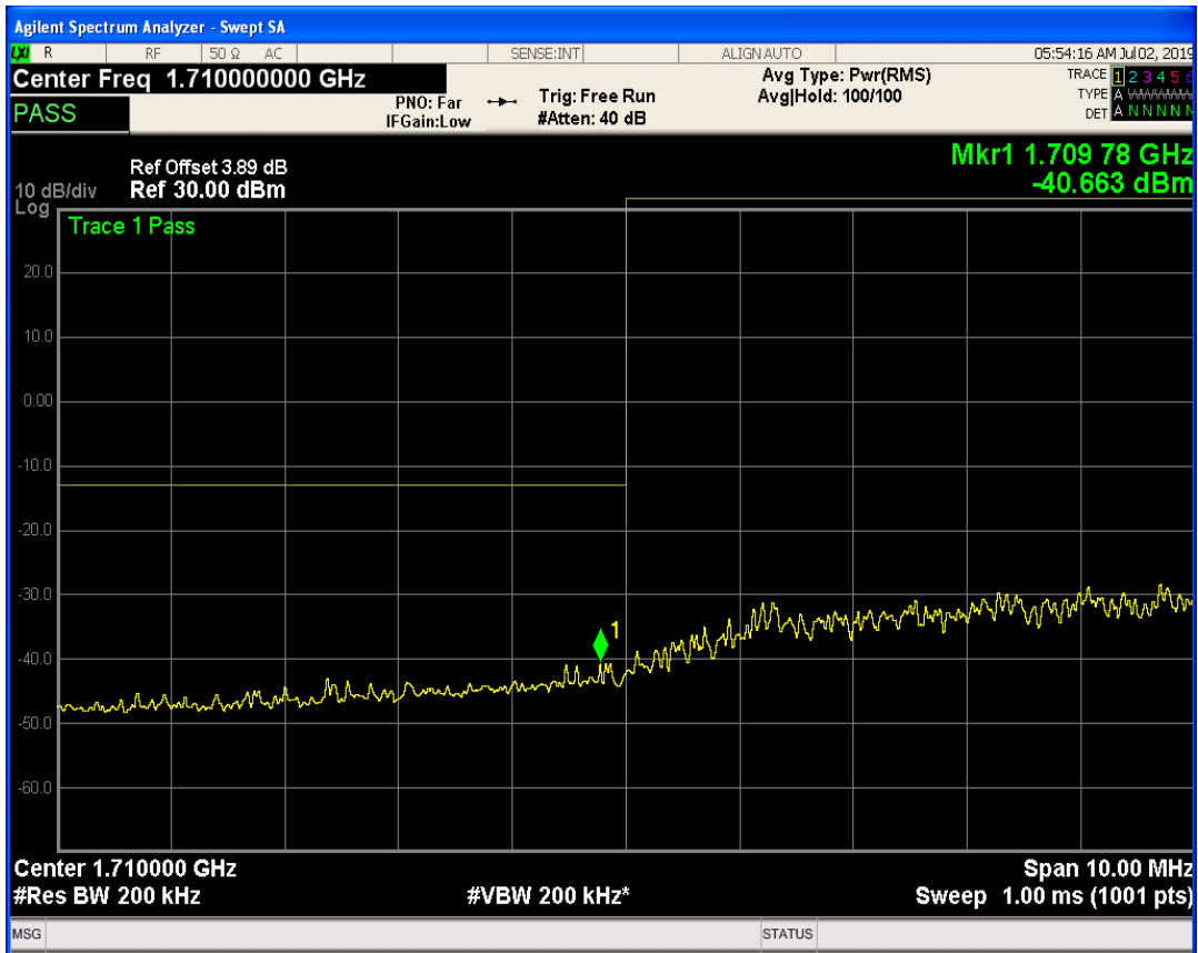
LTE Band4 QPSK BW=20MHz Channel=20050 RB Size=50 Position=#Max
