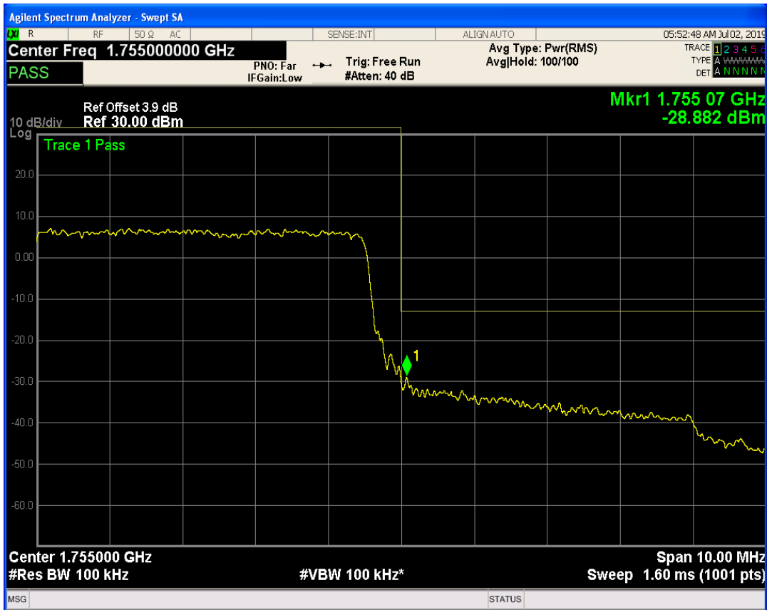
LTE Band4 QPSK BW=10MHz Channel=20350 RB Size=25 Position=#Max
