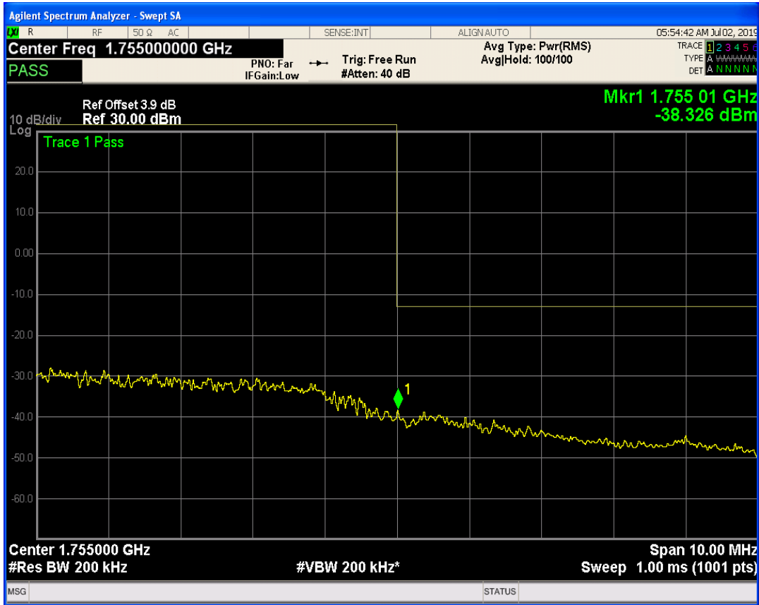
LTE Band4 QPSK BW=20MHz Channel=20300 RB Size=50 Position=#Max
