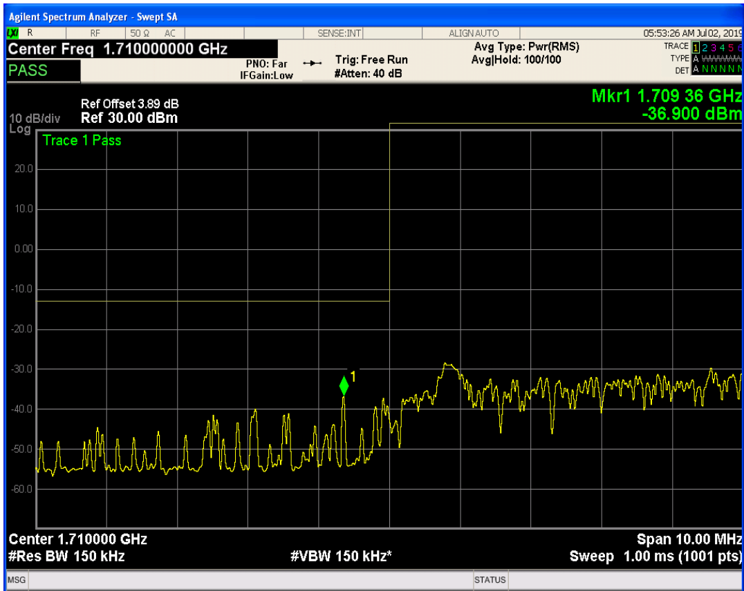
LTE Band4 QAM16 BW=15MHz Channel=20025 RB Size=36 Position=#0
