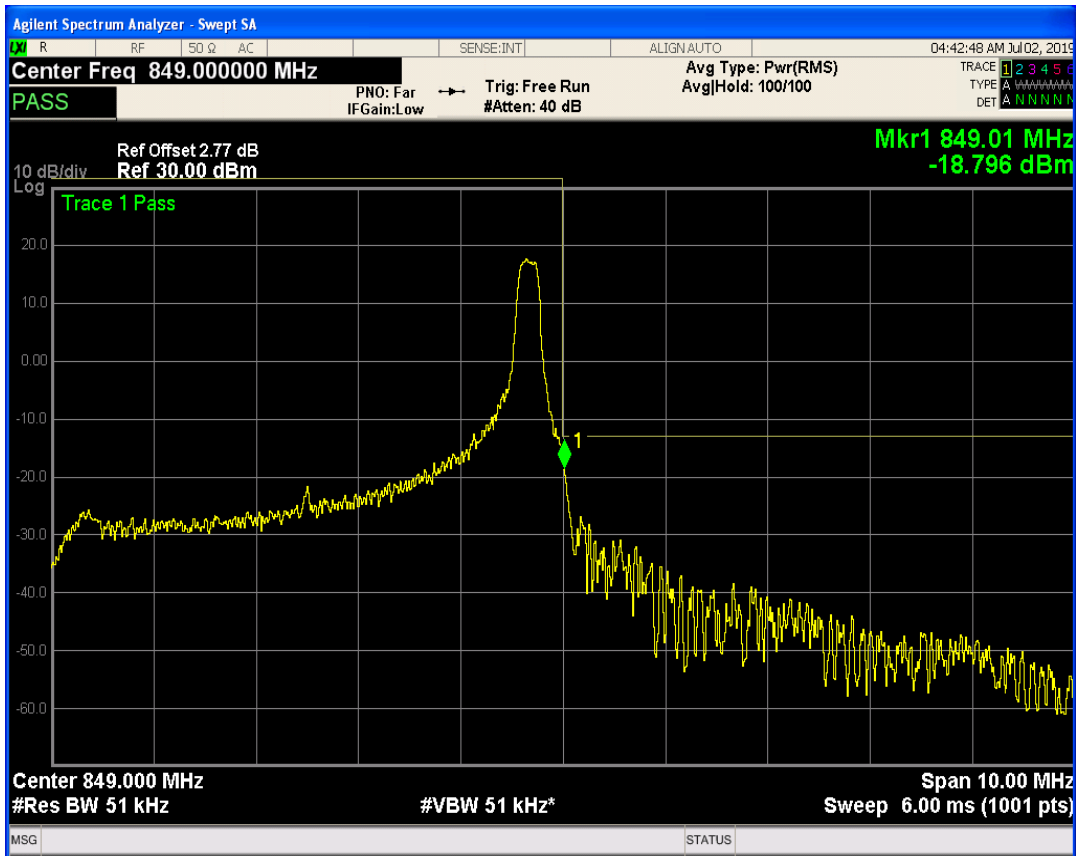
LTE Band5 QAM16 BW=5MHz Channel=20625 RB Size=12 Position=#0
