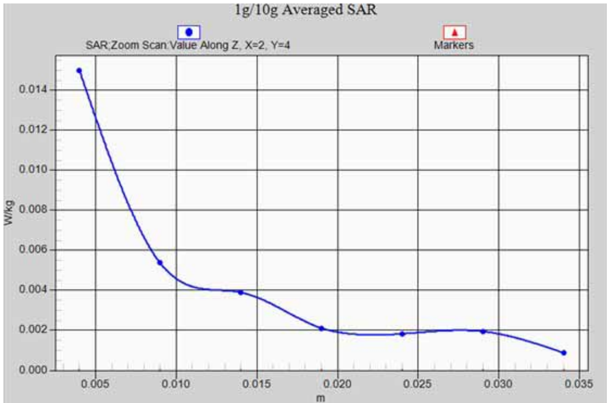
WiFi 802.11b RIGHT/CHEEK-Mid_ z-axis scan
