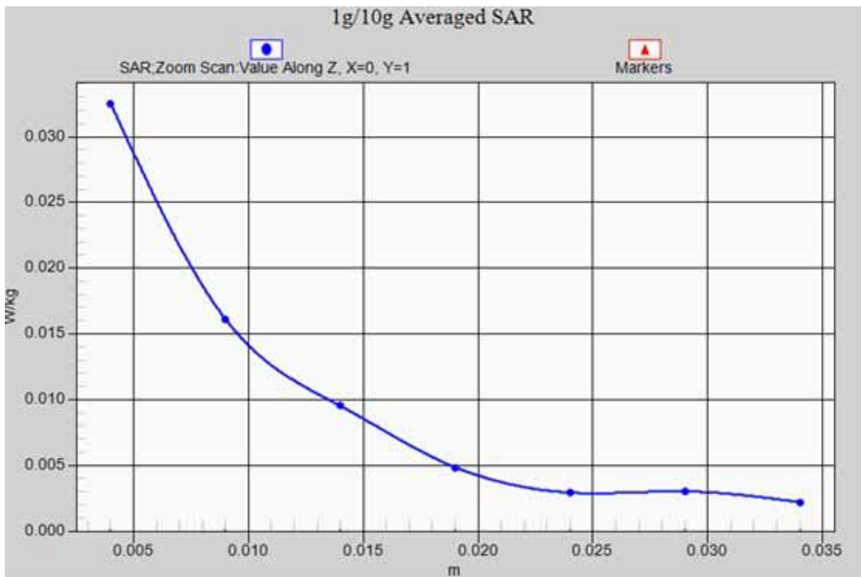
WiFi 802.11b(Body)/Back side-Mid_ z-axis scan
