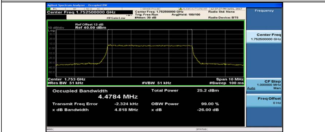
Band4_5MHz_16QAM_20375_25RB#0
