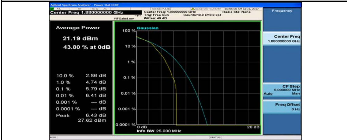
Band2_3MHz_QPSK_18900_1RB#0
