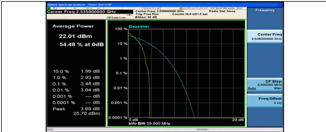
Band7_5MHz_16QAM_21100_1RB#0
