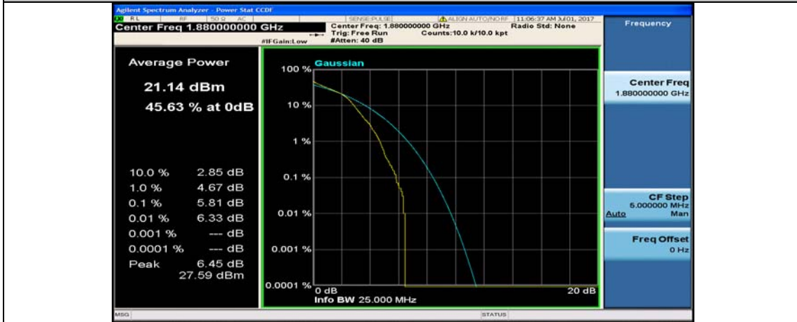
Band2_10MHz_QPSK_18900_1RB#0
