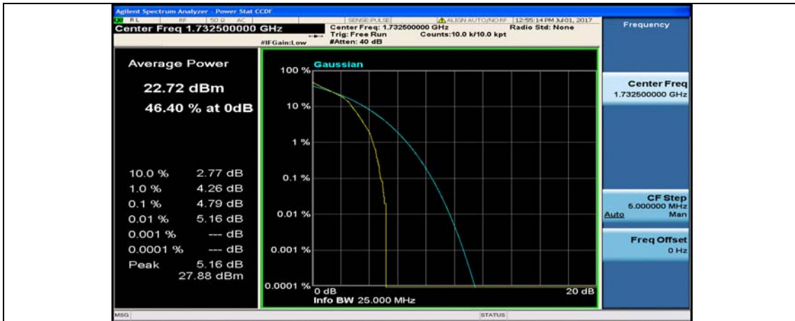
Band4_15MHz_QPSK_20175_1RB#0
