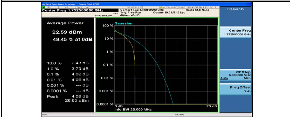
Band4_5MHz_16QAM_20175_1RB#0
