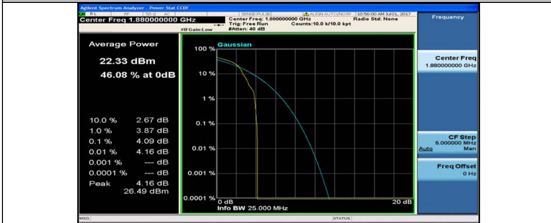
Band2_5MHz_QPSK_18900_1RB#0
