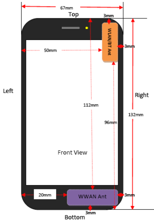
Fig.14.1 EUT Antenna Locations
