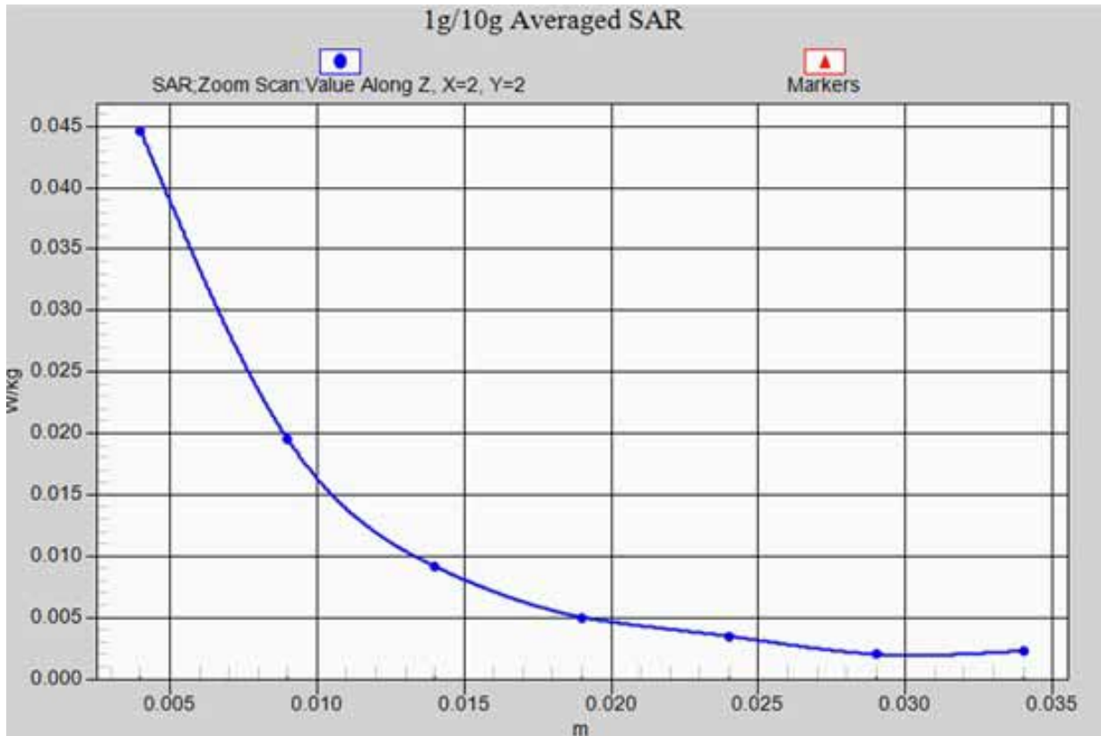
WiFi 802.11b(Body)/Back side-High_ z-axis scan
