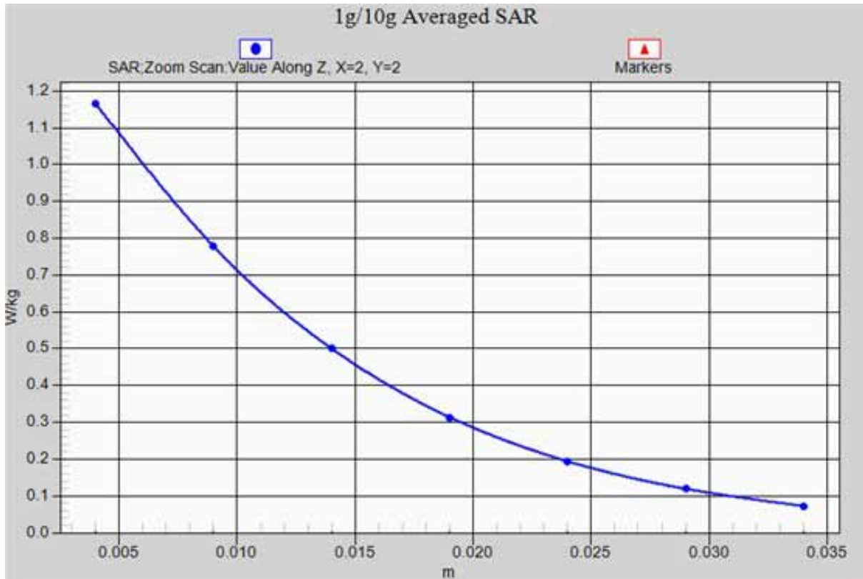
WCDMA Band II- RIGHT/CHEEK-Low_ z-axis scan
