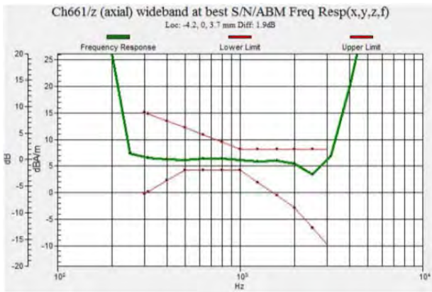
Fig 7.5 GSM1900 Ch661
