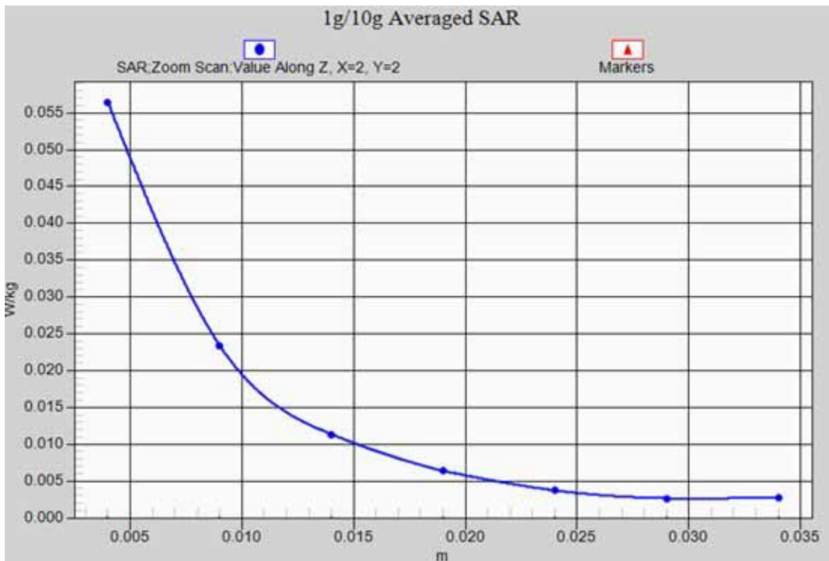
WiFi 802.11b LEFT/TILT-Low_ z-axis scan
