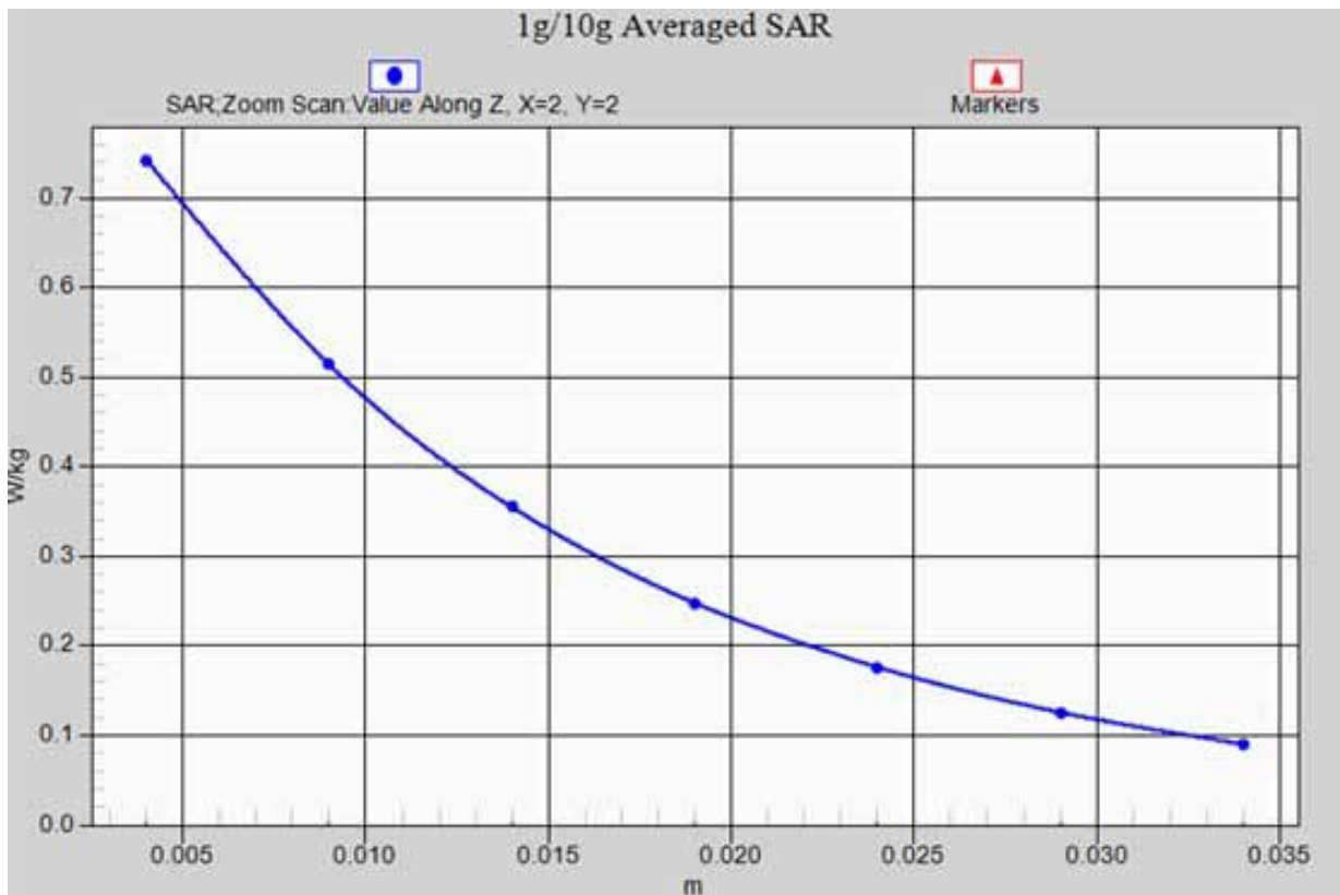
WCDMA Band V(Body)/Back side-Low_ z-axis scan
