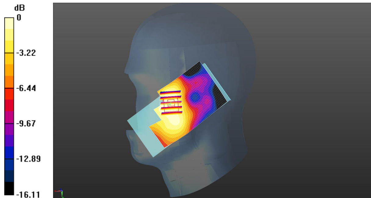
0 dB = 0.0717 W/kg = -11.44 dBW/kg
