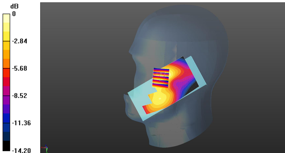
0 dB = 0.0968 W/kg = -10.14 dBW/kg
