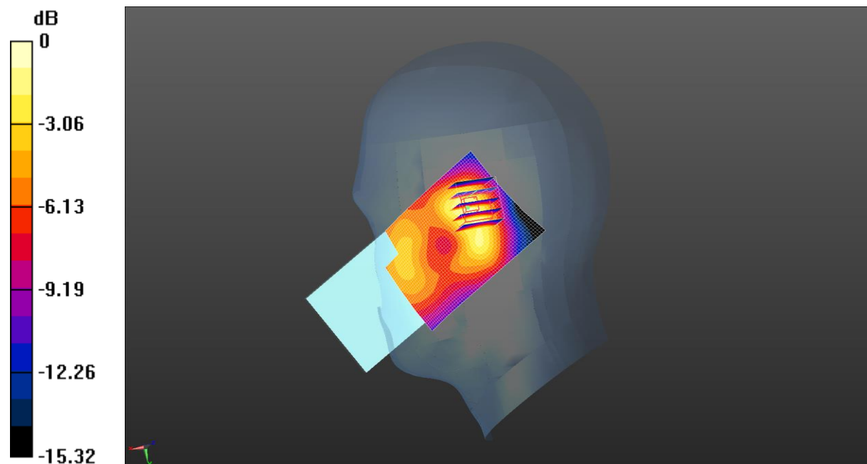
0 dB = 0.0569 W/kg = -12.45 dBW/kg
