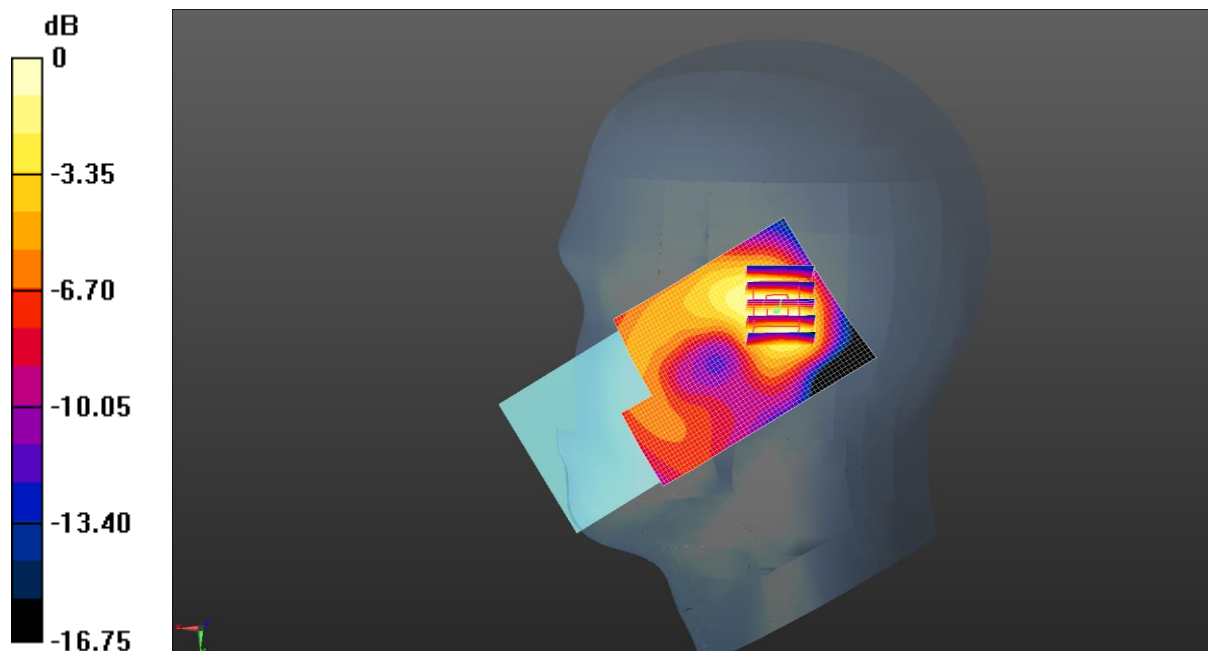
0 dB = 0.0665 W/kg = -11.77 dBW/kg
