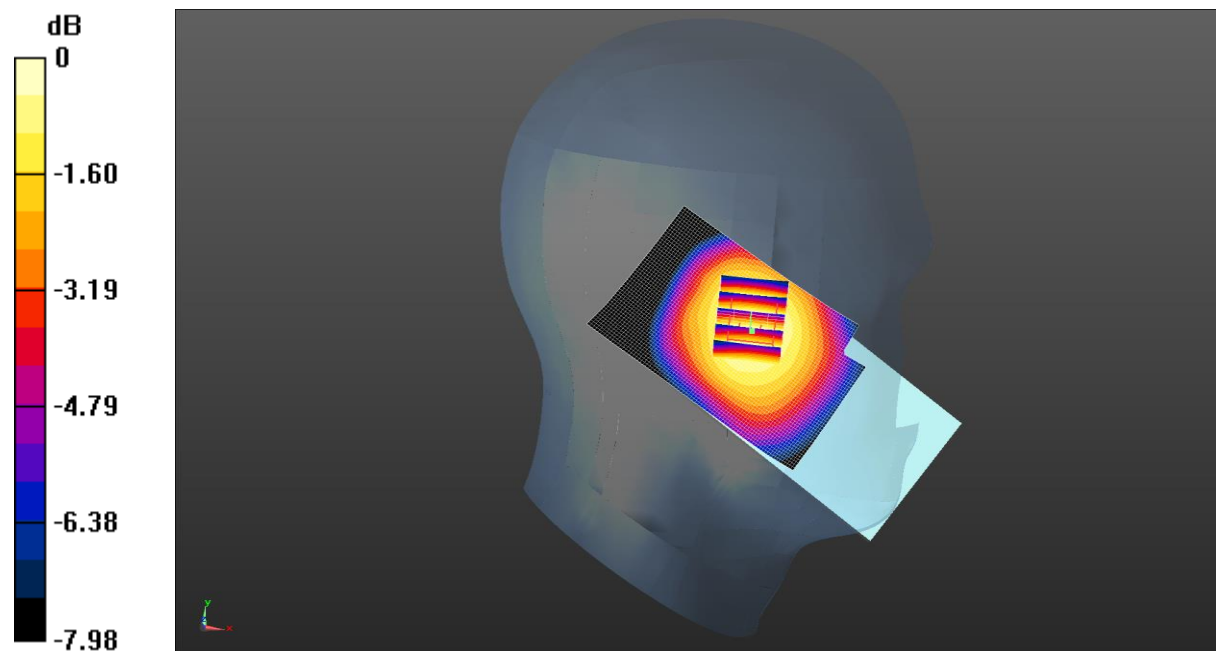
0 dB = 0.0934 W/kg = -10.30 dBW/kg
