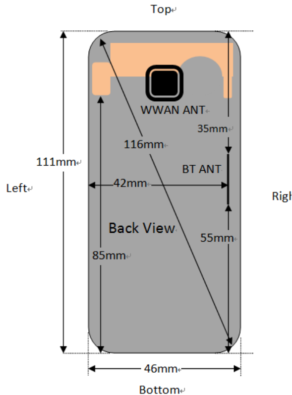
Fig.14.1 EUT Antenna Locations
