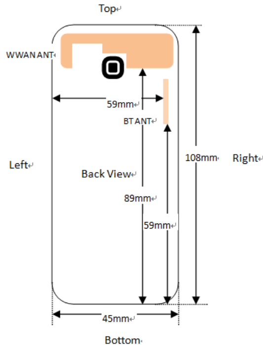
Fig.14.1 EUT Antenna Locations
